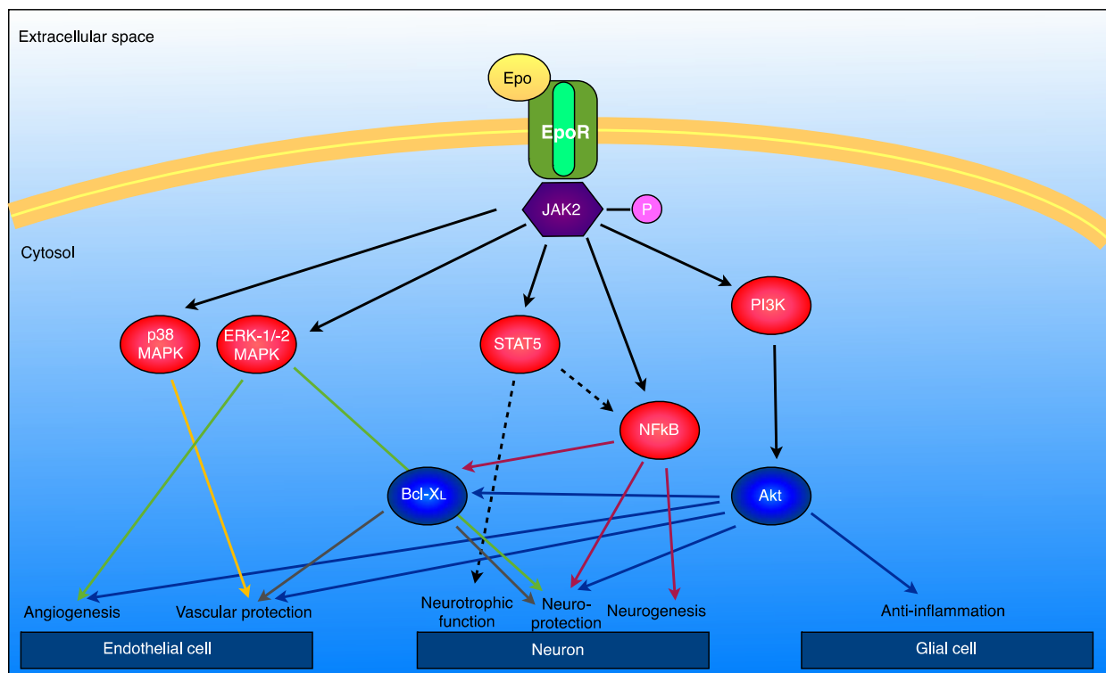
Fig. 3. Epo Signaling
