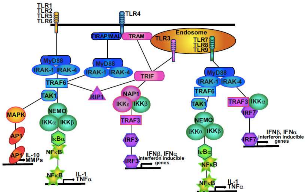
Fig. 6. TLRs signaling
