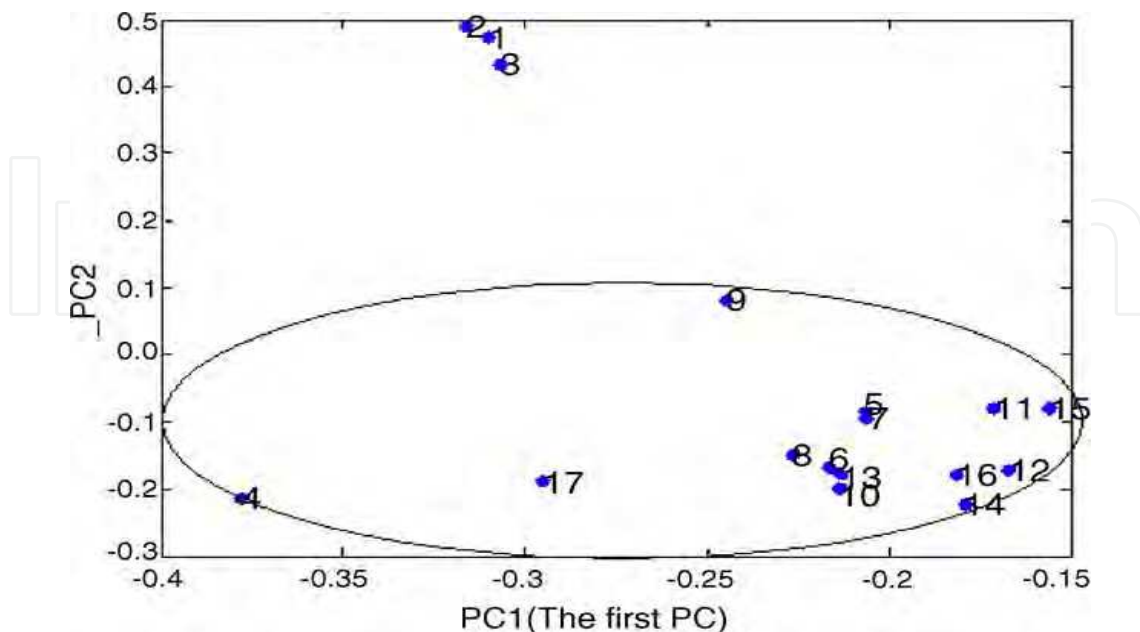
Fig. 4. The score plot obtained by principal components analysis where PC1 means the scores coordinates of principal component 1 and PC2 the ones of principal component 2.
