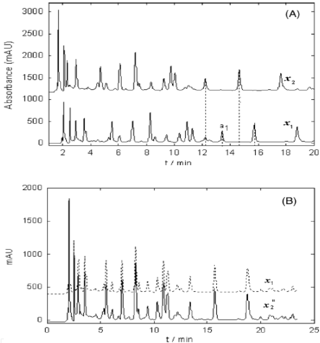
Fig. 7. Comparison of chromatograms X_1 and X_2 measure by the same kind of column but from different companies: X_1 (Agilent Inc.) and X_2 (Waters Inc.). (A) Original chromatograms of samples X_1 and X_2 at wavelength 260nm, respectively. (B) Original chromatograms of samples X_1 and chromatogram X''_2 of sample X_2 after correction of retention time shifting by local least-square technique.
