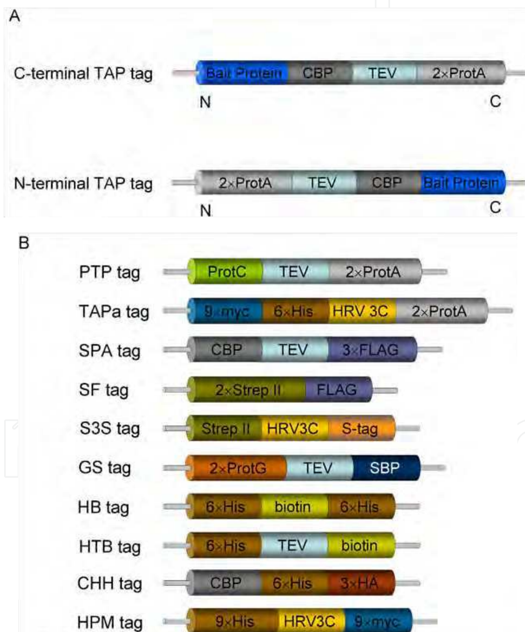
Fig. 1. Diagrammatic sketch of the TAP tag. (A) The original C- and N-terminal TAP tag. (B) Variation of TAP tags developed over the past few years.
