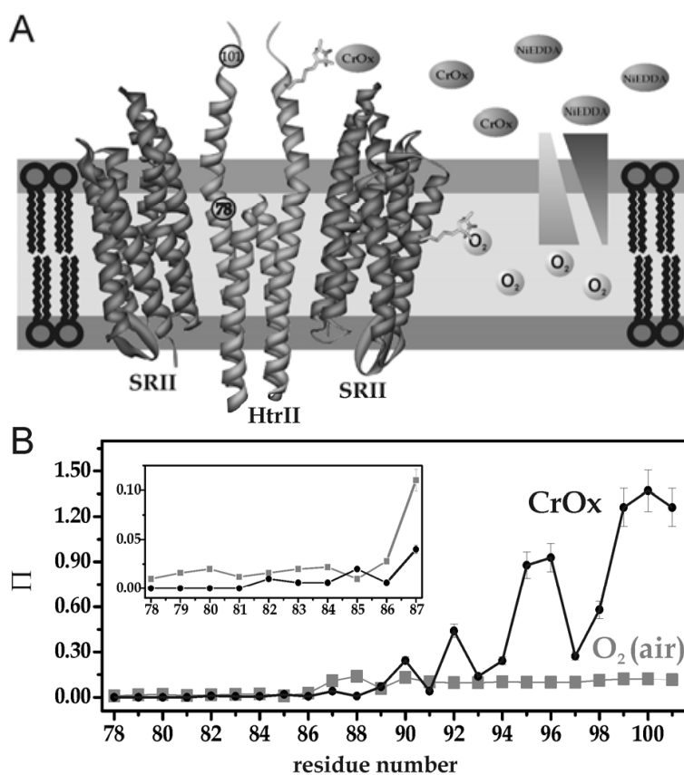
Fig. 4. Spin label accessibilities by power saturation. (A) Structure of the NpSRII/NpHtrII complex in a lipid bilayer (light gray: hydrophobic region, medium gray: headgroup region). The concentration gradients for water-soluble reagents (CrOx and NiEDDA) and lipid-soluble reagents (O 2 ) are indicated by shaded triangles. The first (78) and last residue (101) of the region investigated are indicated. (B) Accessibility parameters \Pi_{CrOx} (black circles) and \Pi_{Oxygen} (gray squares) vs. residue number. \Pi_{CrOx} values have been obtained with 50 mM CrOx, \Pi_{Oxygen} values with air (21% O 2 ). The inset depicts magnified the region from residues 78 to 87 to show the periodicity of 3.6 for \Pi_{CrOx} and \Pi_{Oxygen} .
