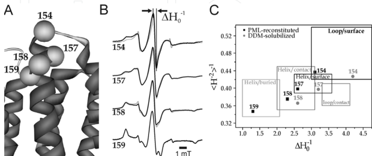
Fig. 3. Mobility analysis of spin labelled proteins. (A) Crystal structure of NpSR II (Luecke et al., 2001). The C \alpha atoms of spin labeled sites are shown as spheres. (B) X band EPR spectra of spin labeled NpSR II solubilised in detergent (gray) or reconstituted in purple membrane lipids (black). (C) Two-dimensional mobility plot of the inverse of the second moment vs. the inverse of the central linewidth (solubilized: gray circles, reconstituted: black squares), determined from the spectra in B. Boxes indicate the topological regions of proteins according to Isas et al. (2002) and Mchaourab et al. (1996).
