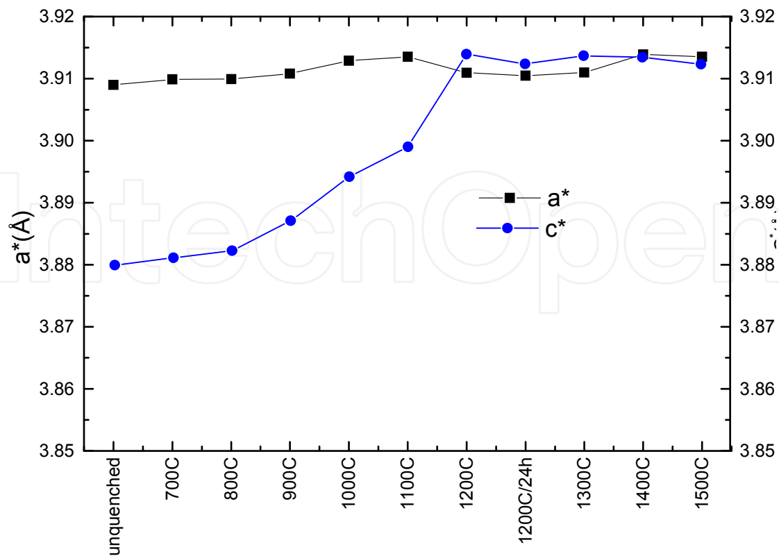
Fig. 7. Lattice parameters of \text{La}_{0.6}\text{Sr}_{0.4}\text{FeO}_3 vs. quenching condition.
