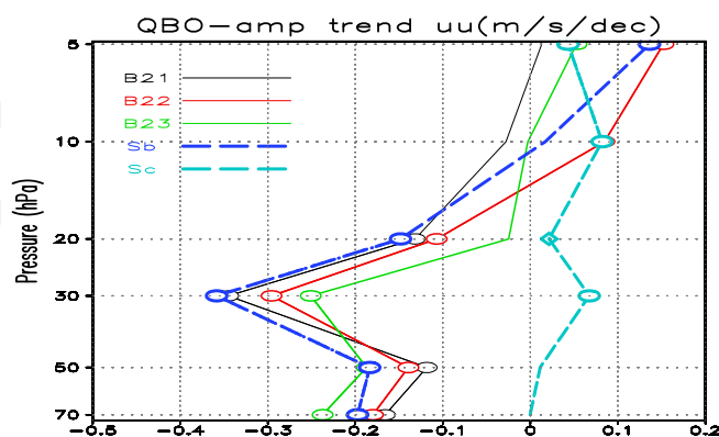
Fig. 19. Trends of the QBO amplitude. Vertical profiles of the linear trends ( \text{ms}^{-1} per decade) in the QBO amplitude for the zonal-mean zonal wind (averaged from 10^{\circ}\text{S} to 10^{\circ}\text{N} ) from 70 to 5 hPa in all simulations. Open circles and diamonds represent the trend being different from zero at the 99% and 95% confidence levels ( t -test), respectively. The QBO amplitude was calculated by the direct method.
