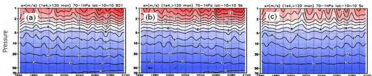
Fig. 7. Low-frequency residual vertical velocity. Time-pressure cross section of the low frequency (period longer than 120 months) component of the residual vertical velocity (averaged between 10°S and 10°N) from 70 to 1 hPa. Units are 10^{-4} ms -1 .
