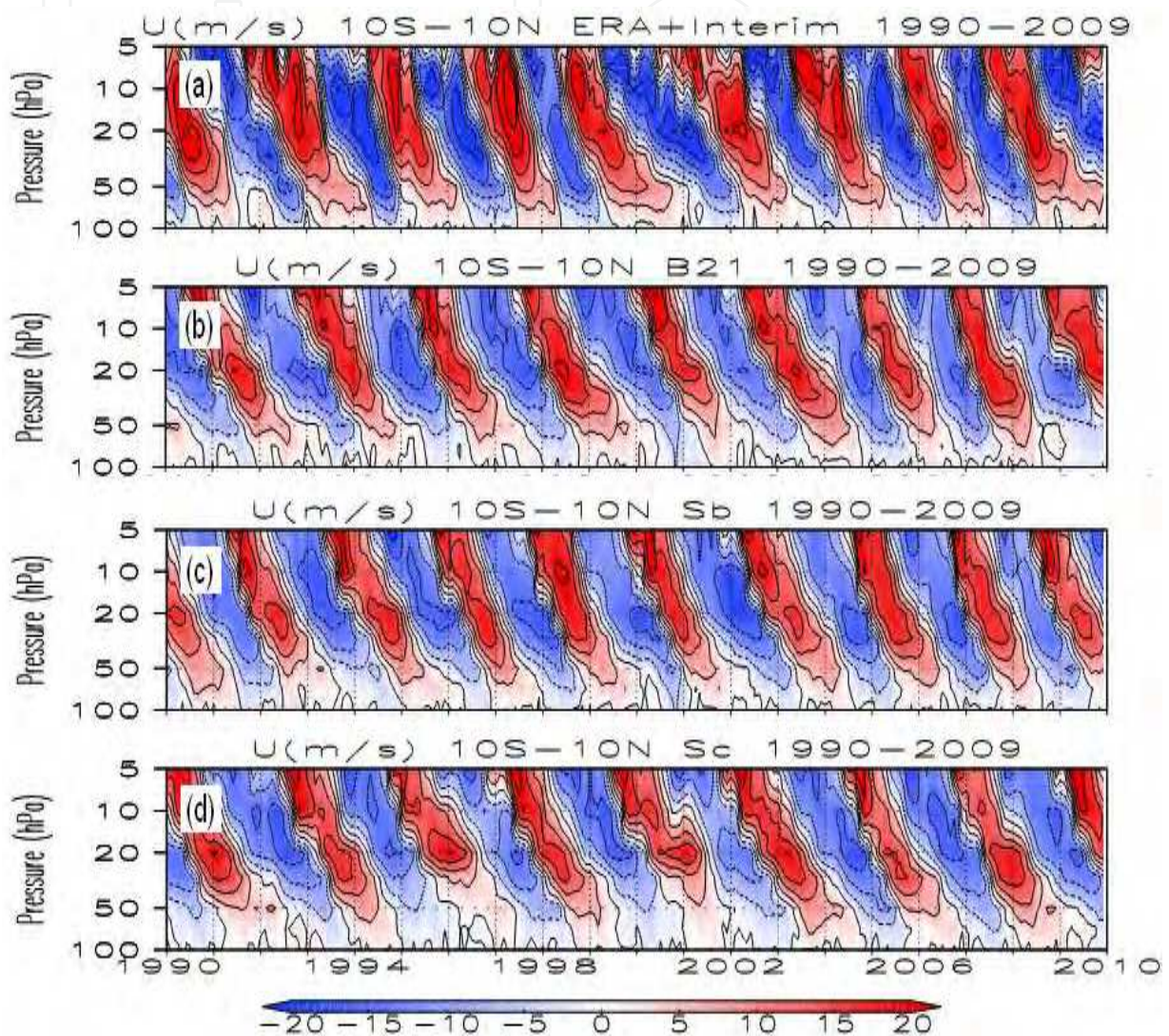
Fig. 9. Zonal wind evolution in the tropics. Evolution of zonal-mean zonal wind (averaged between 10°S and 10°N) from 100 to 5 hPa for the 20 years from 1990 to 2009: (a) ERA-Interim, (b) B21, (c) Sb, and (d) Sc.
