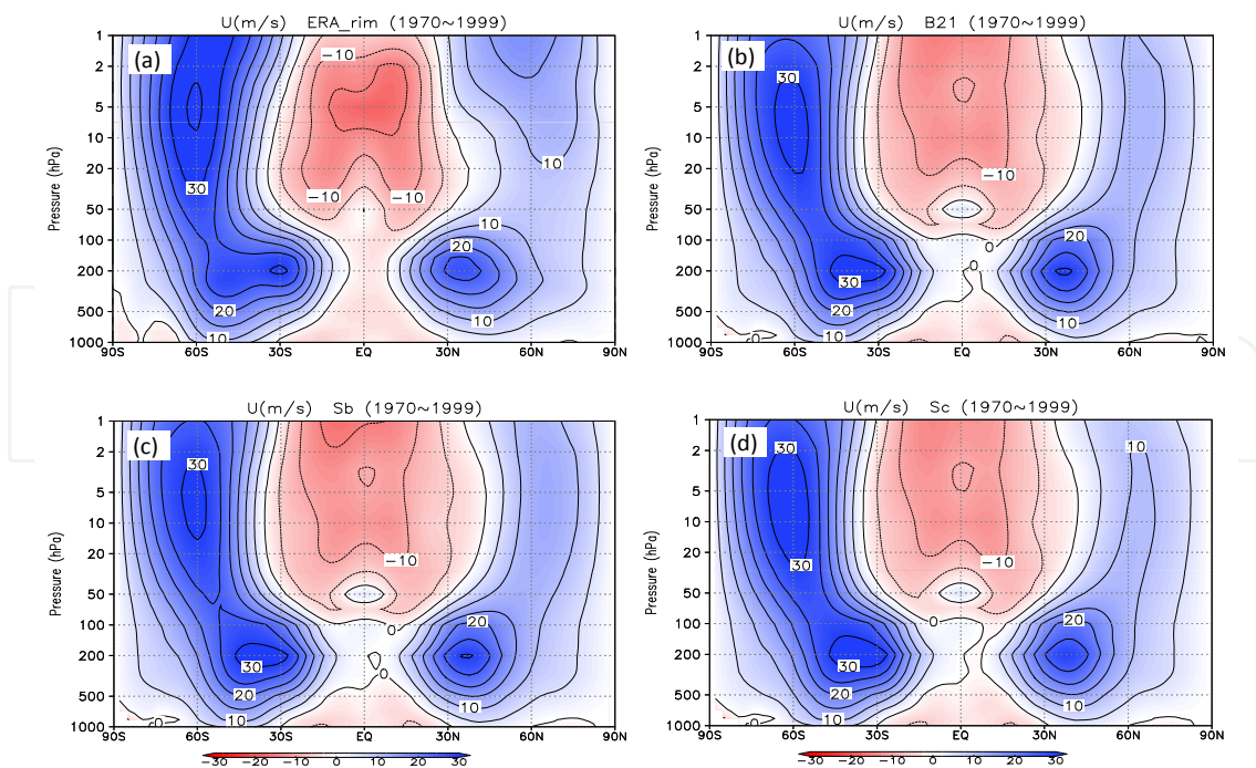
Fig. 3. Annual- and zonal-mean zonal wind. Same as Fig.2 except for zonal wind ( \text{ms}^{-1} ). The contour interval is 5 \text{ms}^{-1} , and blue colors represent positive (westerly) winds and red colors negative (easterly) winds.
