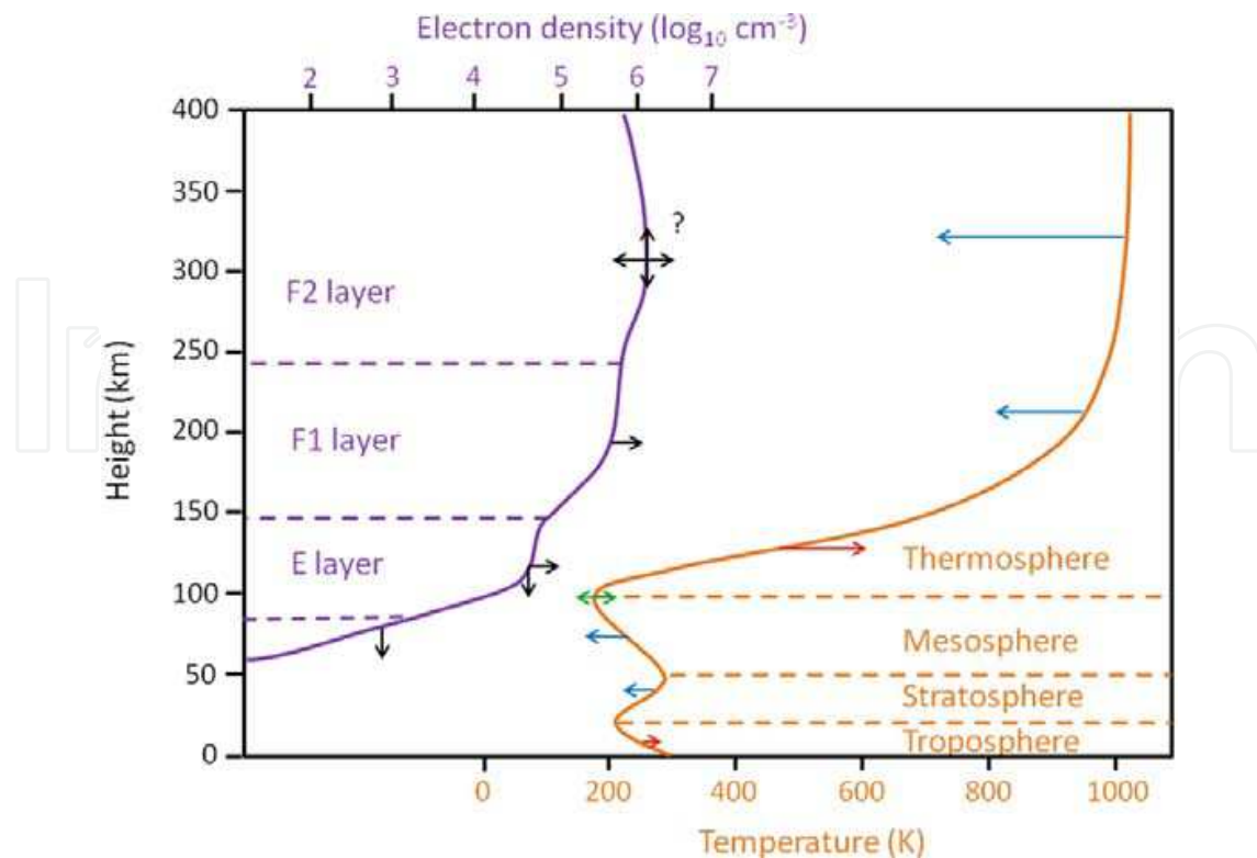
Fig. 1. Schematic summary of observed global mean trends in the atmosphere, after Laštovička et al. (2006a). Changes in the temperature profile (orange) are indicated by red (warming), blue (cooling) and green (no clear trend) arrows. Changes in the electron density profile (purple) are indicated by black arrows. Vertical arrows indicate the movement of the height of the peak electron density of the layer, while horizontal arrows indicate changes in the peak electron density itself. Trends in the F 2 layer vary strongly with location, season, and local time, so that no meaningful global mean can be defined. They are further discussed in section 2.4.
