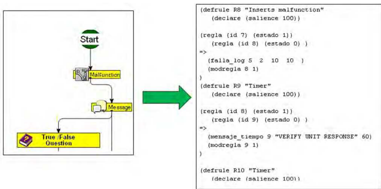
Fig. 10. Knowledge representation in CLIPS.
