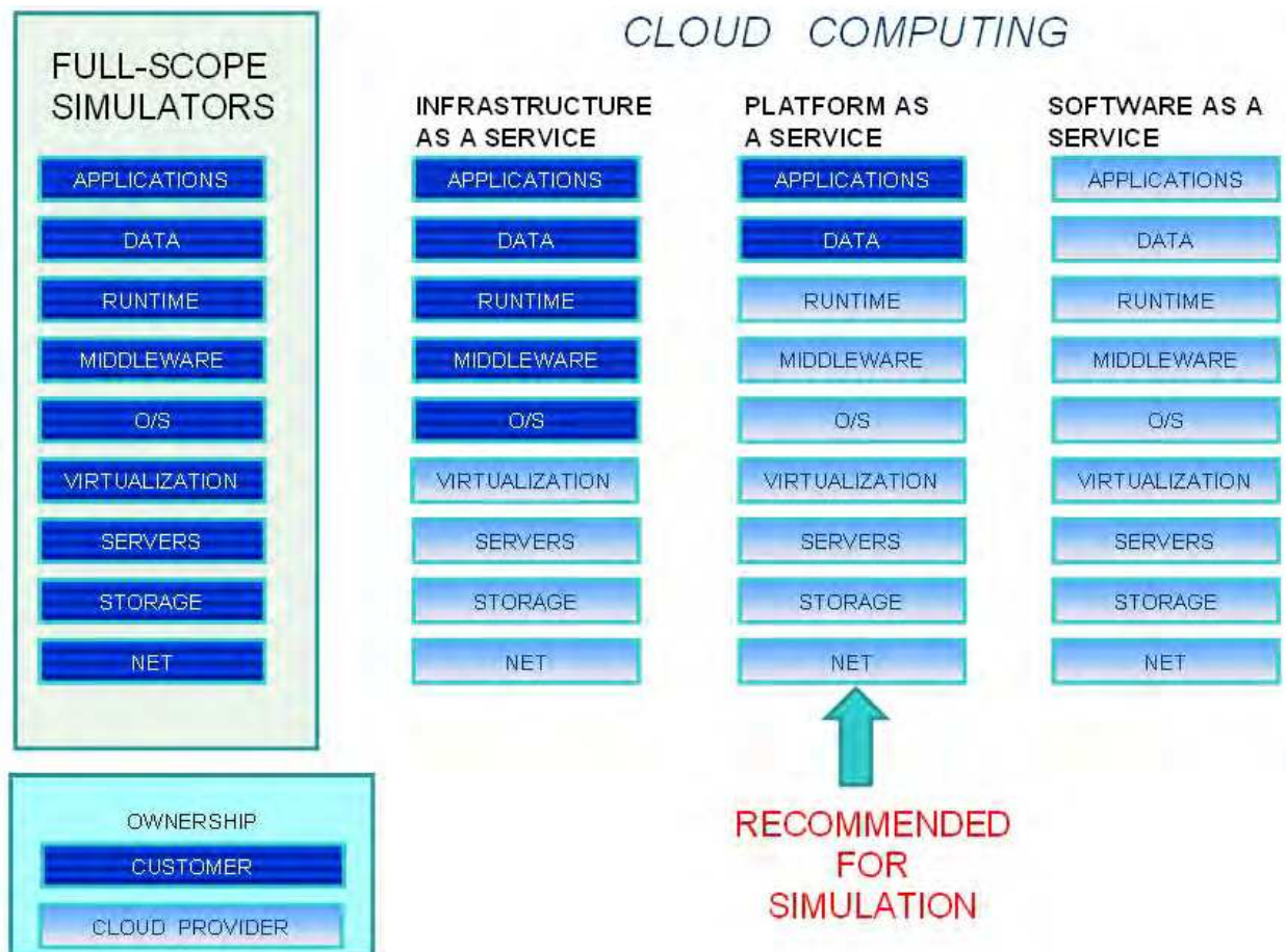
Fig. 6. Cloud computing services.
