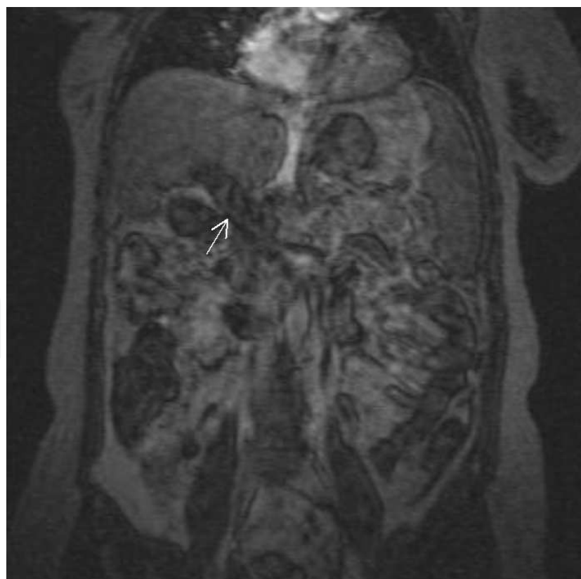
Fig. 9 and 10. The same case - angio-MRI sequence. Inhomogeneous signal of the portal vein with chronic thrombosis.
