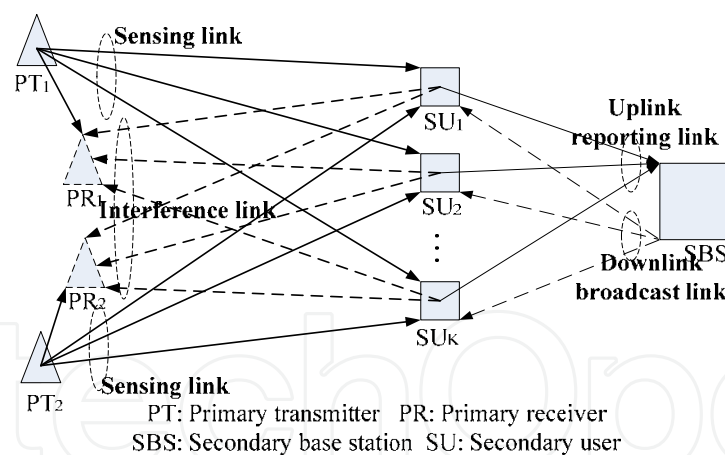
Fig. 1. System model of CRN
