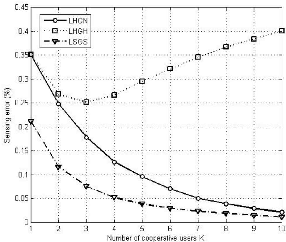
Fig. 2. Sensing performances versus number of cooperative users
