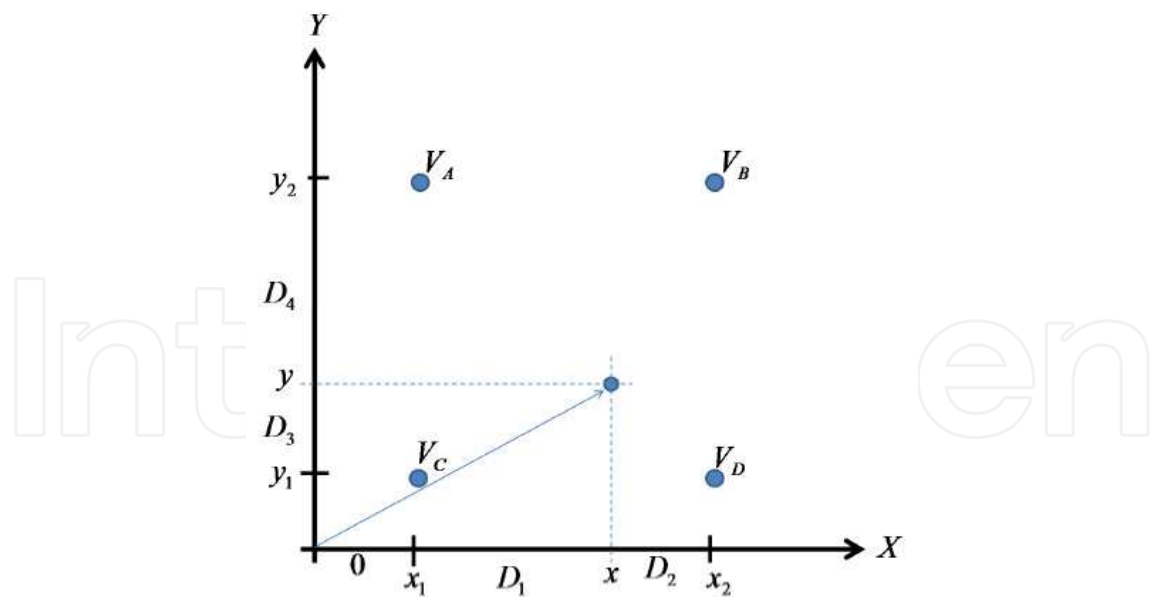
Fig. 10. Scheme to describe the process of event detection. In the Cartesian system position identifies the four voltage signals, V_A , V_B , V_C and V_D , and the position (x, y) of gamma photon interaction on the crystal
