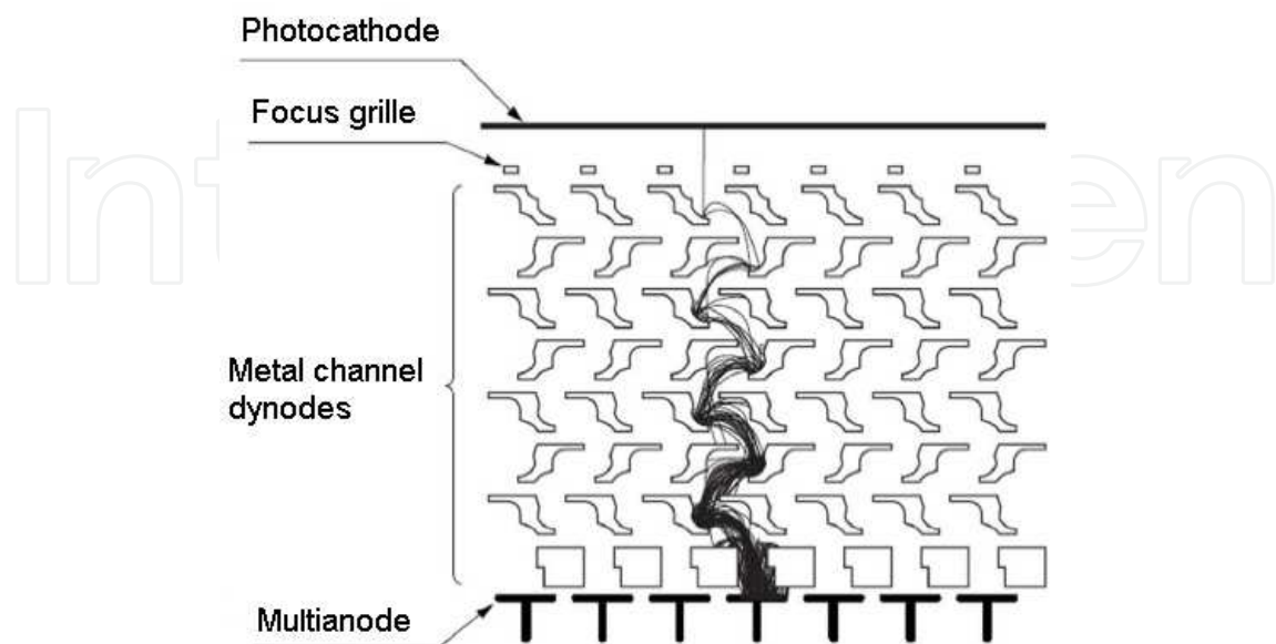
Fig. 7. Dynode structure and electrons trajectory
