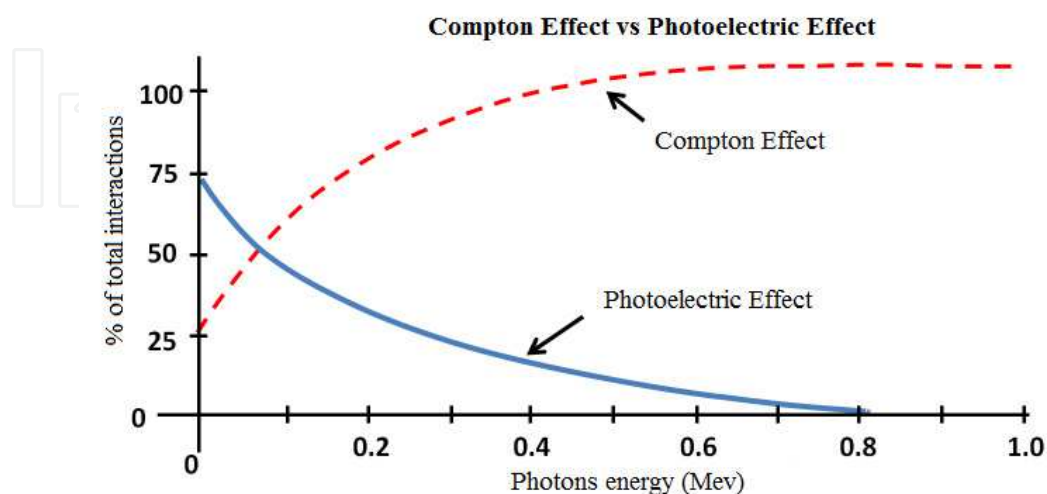
Fig. 4. With very low photon energies, the photoelectric effect is dominant. The Compton effect becomes dominant from 0.1 to 0.15 MeV and onwards
