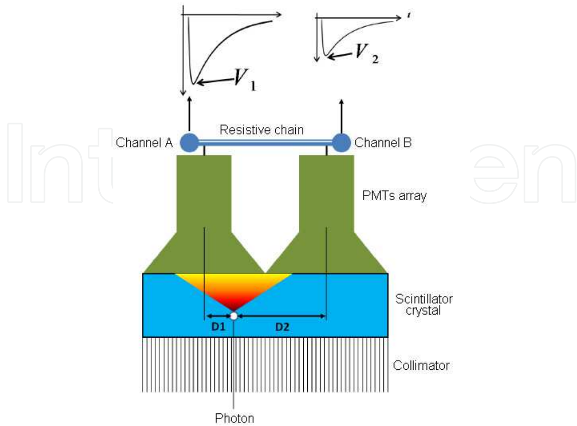
Fig. 9. Illustration of gamma radiation interacting with the photomultiplier tube
