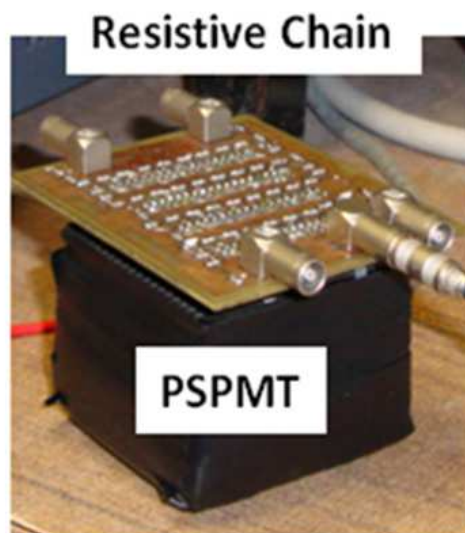
Fig. 13. Scintillator structure coupled with the resistive chain
