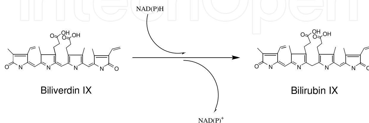
(BVR Reaction)
