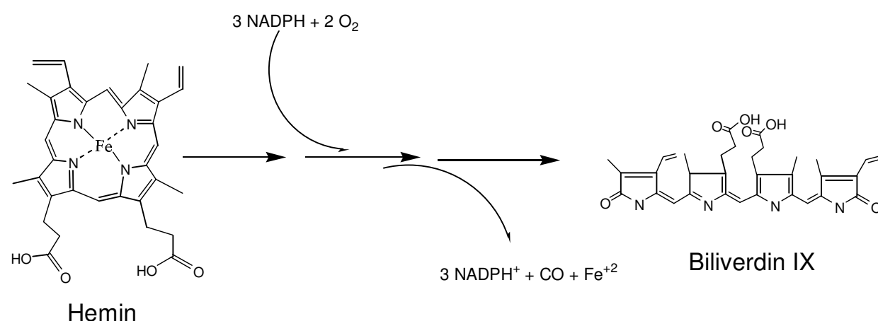
(HO Reaction)
