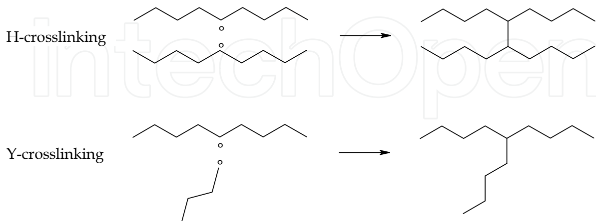
Fig. 1. Reaction of H- and Y- crosslinking.
