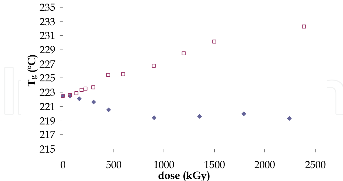
Fig. 6. Change in T_g for PES submitted to electron beam irradiation at room temperature (◆) or 230°C (□) (Li et al., 2006).
