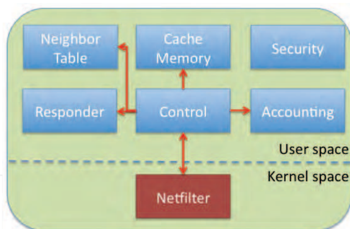
Fig. 6. Internal modules of a content router.
