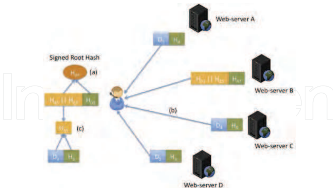
Fig. 10. Parallel data verification scenario. (a) First, the application retrieves the RH and verifies the digital signature. (b) The application retrieves ADs and subsequent data blocks from multiple sources. (c) Data blocks are verified using the previously received ADs.
