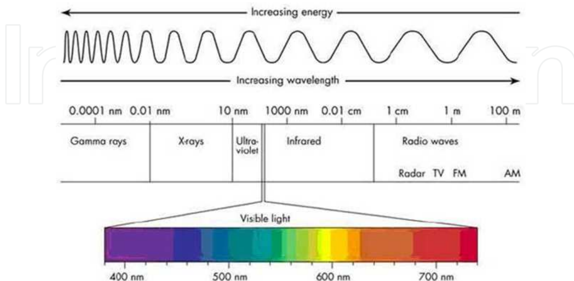
Fig. 1. Electromagnetic wavelength
