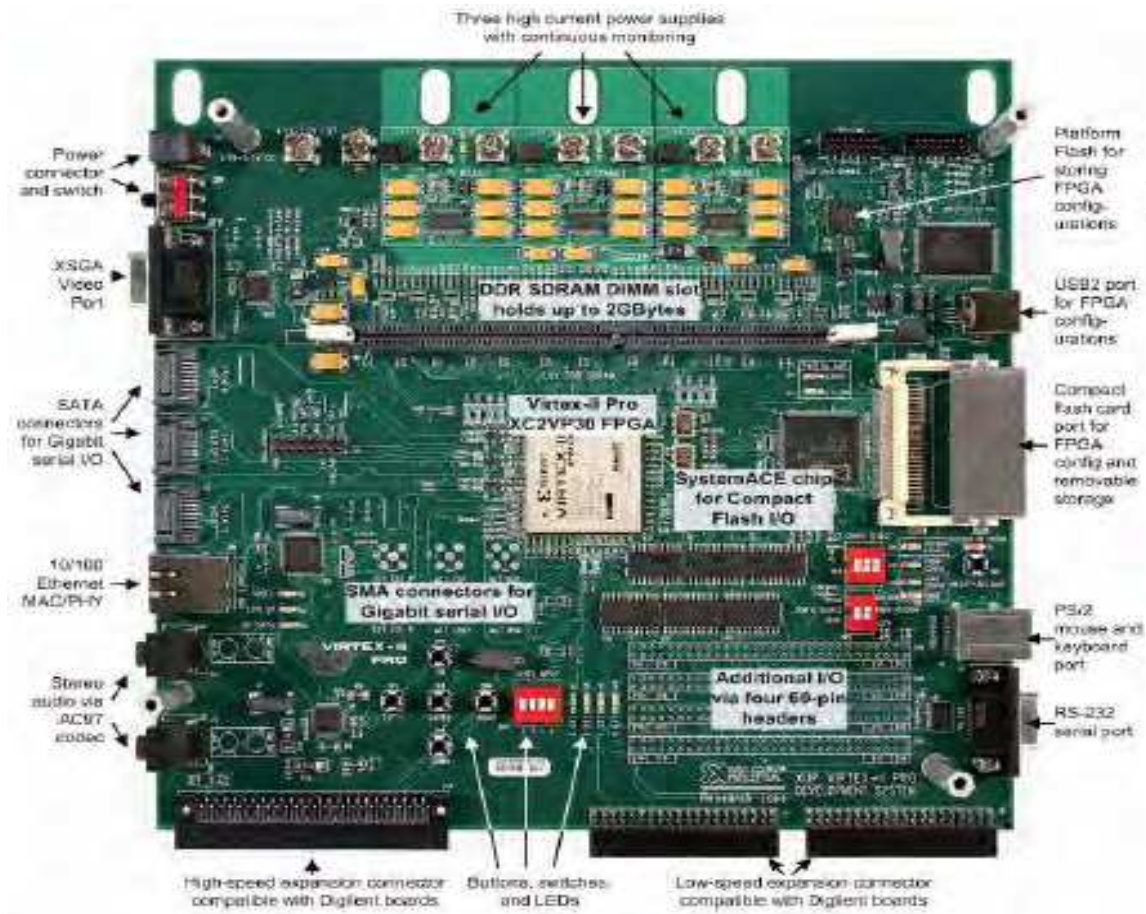
Fig. 18. XUP Xilinx Virtex-II Pro embedded platform.
