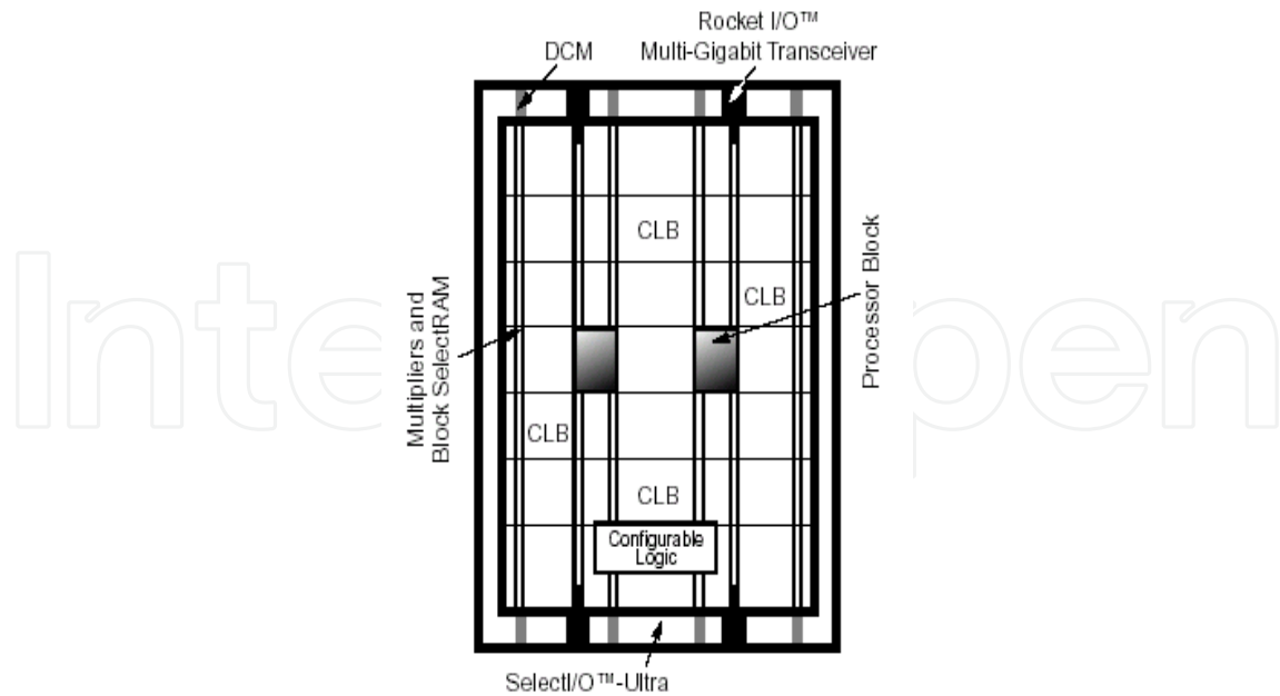
Fig. 12. Overview of the Xilinx Virtex II FPGA chip [Xilinx2, 2007].
