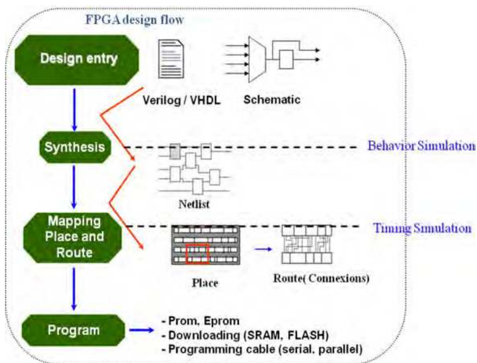
Fig. 14. FPGA design flow overview.
