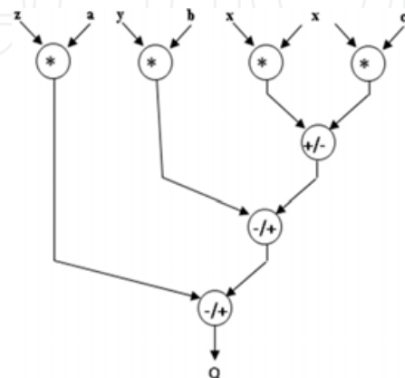
Fig. 16. RTL architecture of the Q functional units.
