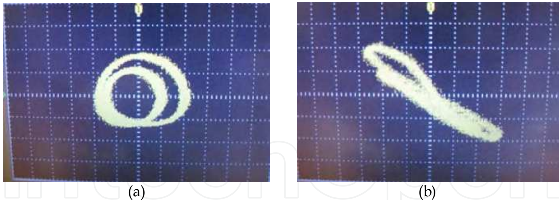
Fig. 22. Real-time measurement results of (a) the (x-y) chaotic attractor, and (b) the (x-z) chaotic attractor.
