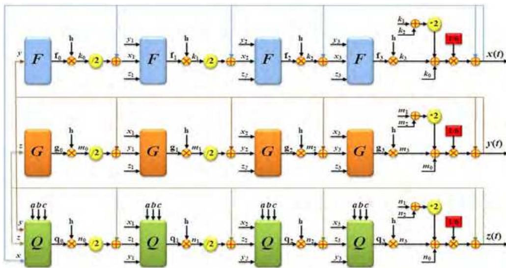
Fig. 15. RTL architecture of the Genesis-Tesi chaotic system.
