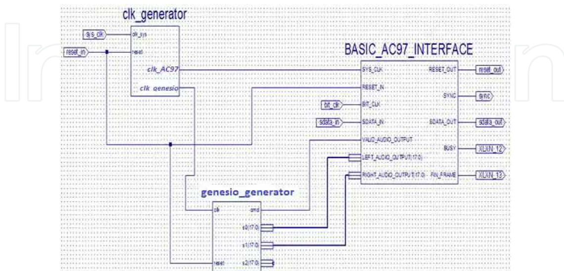
Fig. 20. Functional blocks implemented in the FPGA chip.
