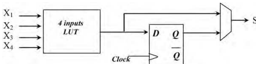
Fig. 10. Generic overview of a 4-input Look-Up Table.
