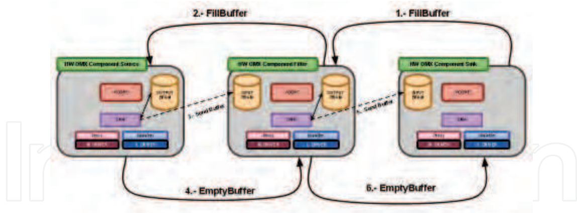
Fig. 11. Sequence of messages in Hw-to-Hw Tunneled Communication
