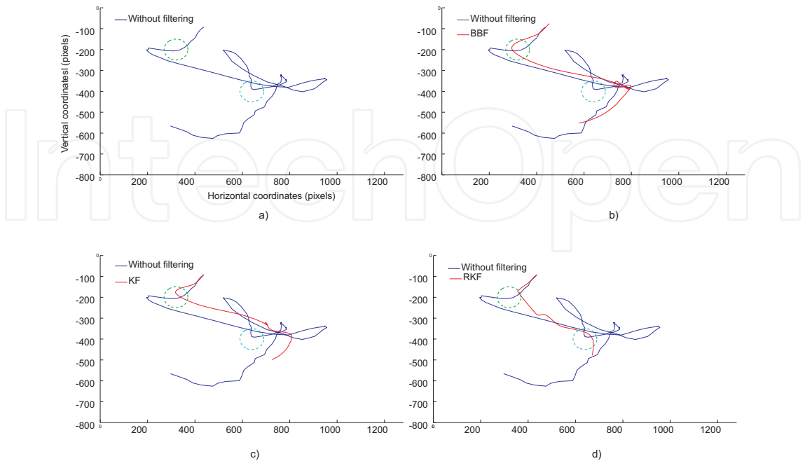
Fig. 15. Pointer path a) without filtering b) with BBF c) with KF d) with RKF
