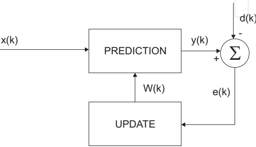
Fig. 10. Block diagram of adaptive filtering implementation
