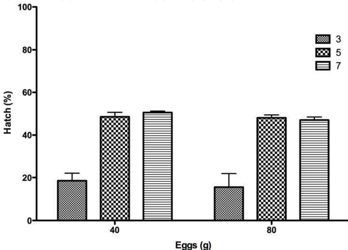
Fig. 1. Hatch rates of wels catfish eggs fertilized with cryopreserved sperm. Each batch of eggs (40 or 80 g) was fertilized with one 5-ml straw of cryopreserved sperm. Columns indicate cooling times employed during cryopreservation (3, 5 or 7 minutes). Data are presented as Mean \pm SD (N = 3).
