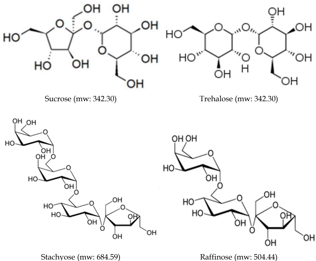
Fig. 6. Sugar structure
