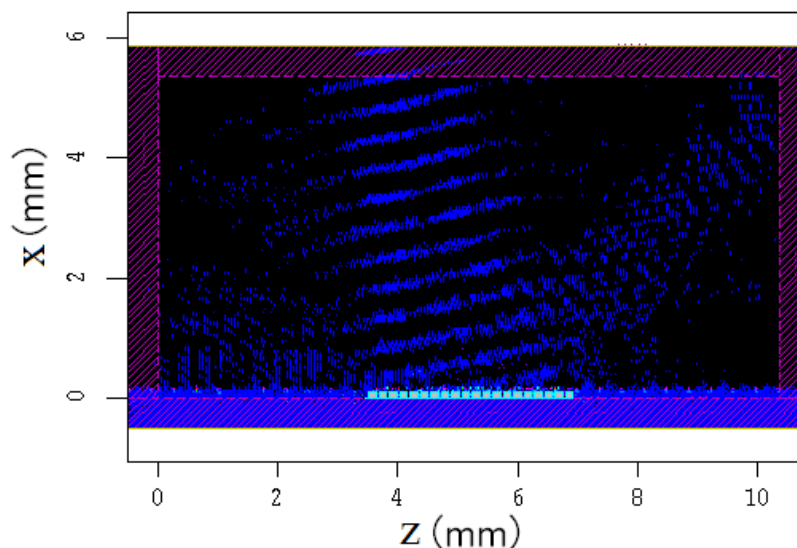
Fig. 11. Contour plot of B_y for superradiant radiation.
