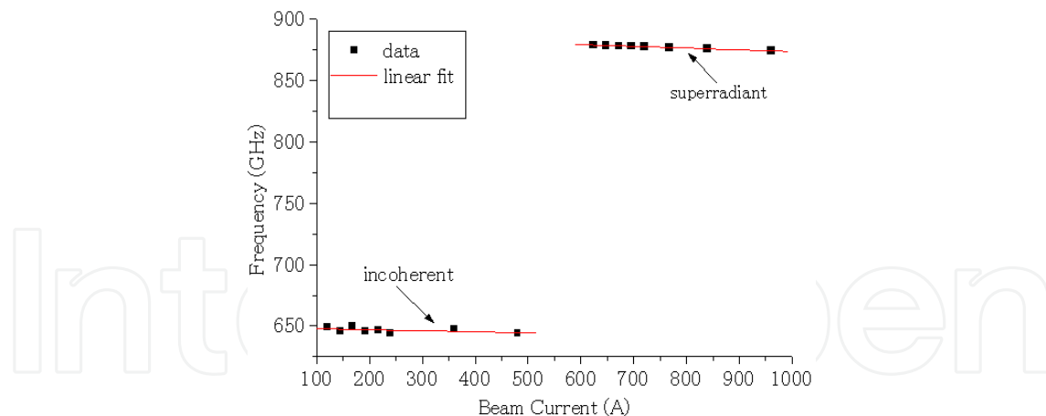
Fig. 13. Frequencies of incoherent and superradiant radiation with respect to beam current.
