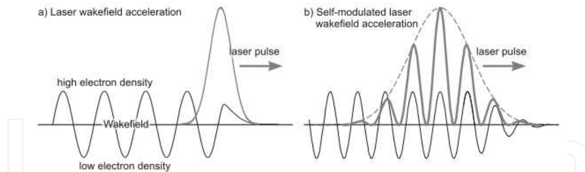
Fig. 2. Laser envelope and electron density schematic in the laser wakefield regime (a) and in the self-modulated wakefield regime.
