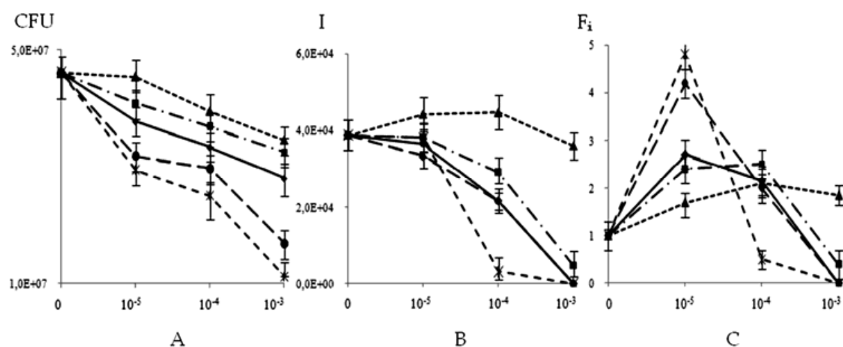
Fig. 5. E.coli recA'::lux strain response on AR action (horizontal axis - concentration, M): the number of survived cells (A), the absolute intensity of bioluminescence (B), the relative value of induction index of SOS-response (C). -▲- - C_1\text{-AR} , -■- - C_3\text{-AR} , -●- - C_5\text{-AR} , -●- - C_6\text{-AR} , -*- - C_{12}\text{-AR} .
