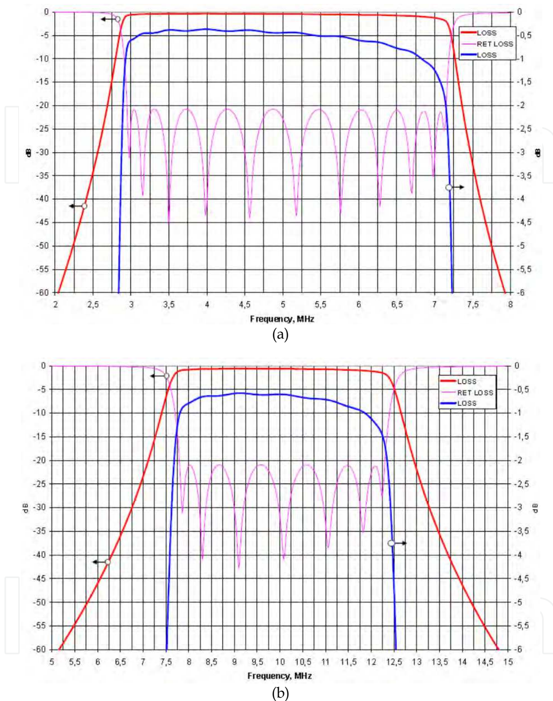
Fig. 12. Performance data of the (a) 5 MHz and (b) 10 MHz 100 W band-pass filters.
