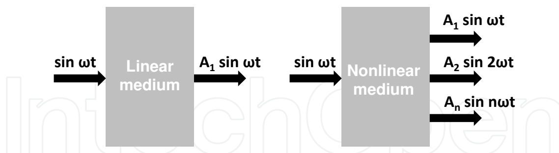
Fig. 11. Linear and nonlinear wave propagation in solid materials.
