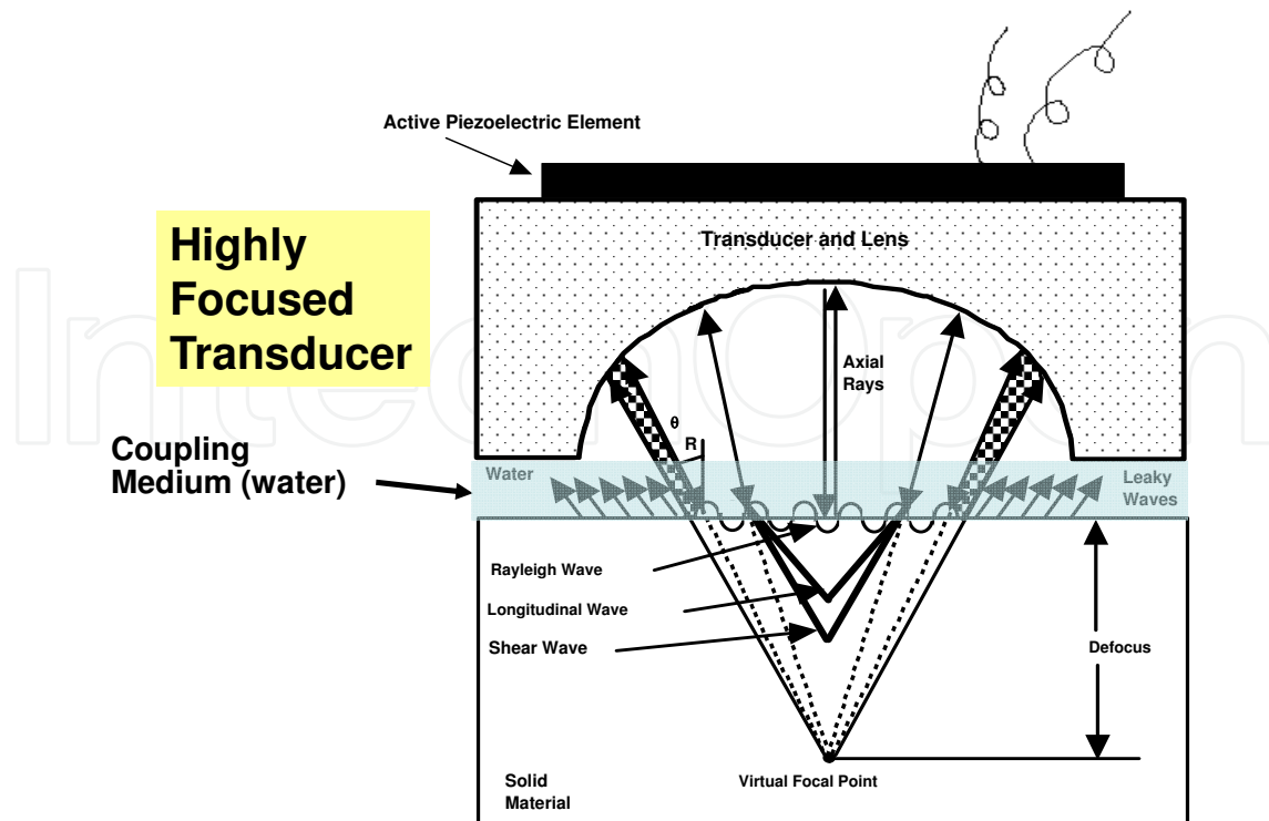
Fig. 8. Principle of ultrasonic microscopy.
