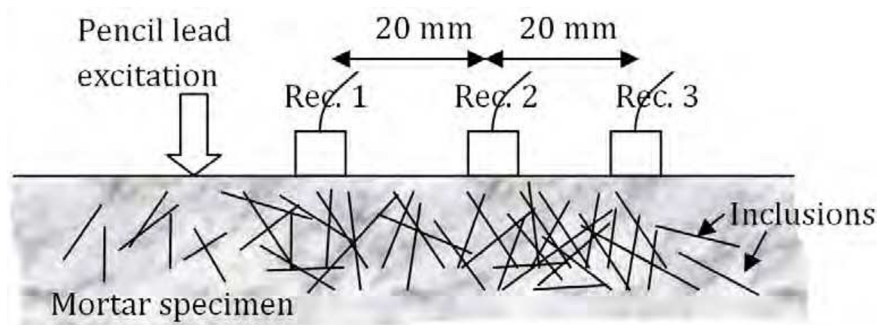
Fig. 1. The experimental setup.
