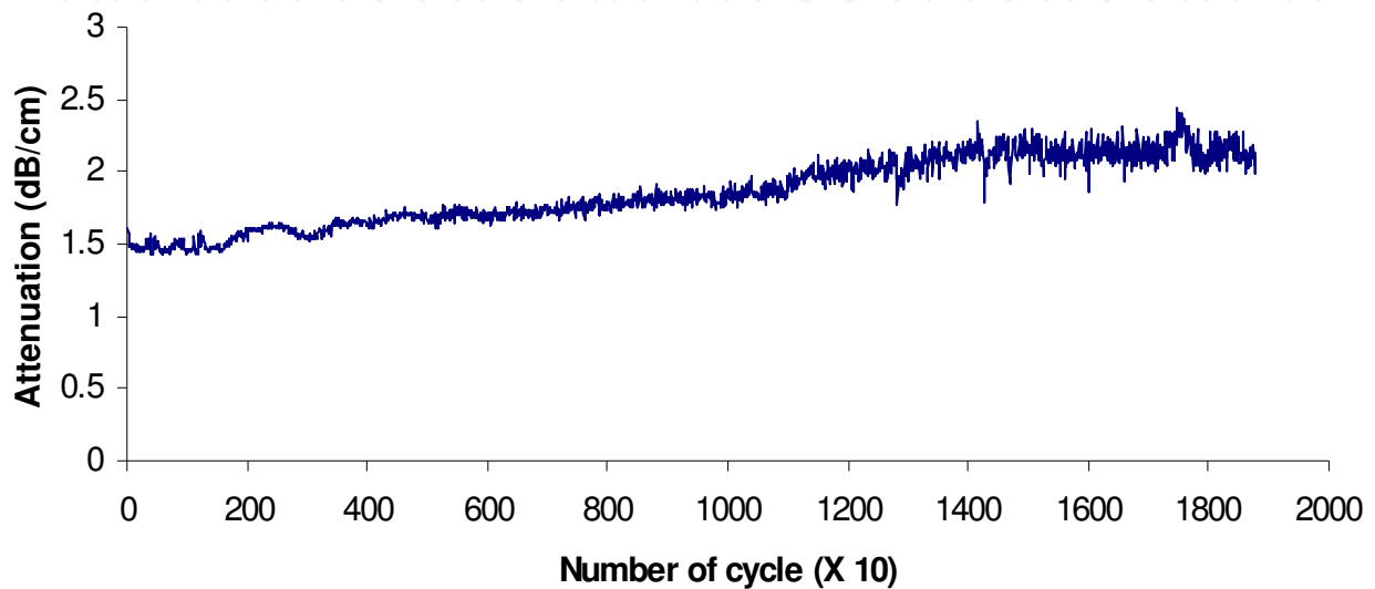
Fig. 16. Variation of ultrasonic attenuation with fatigue life
