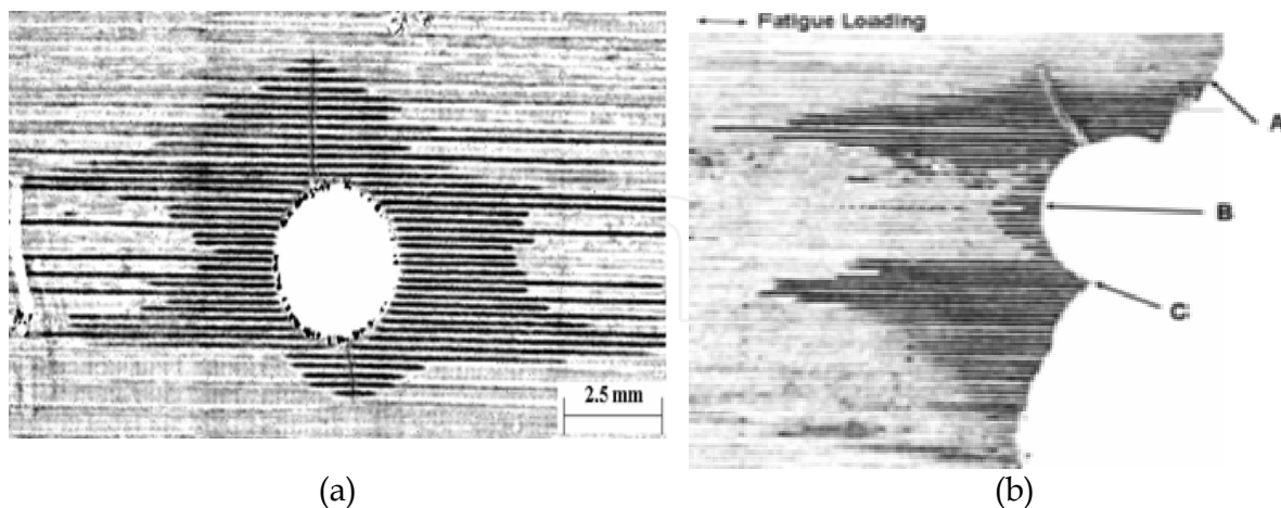
Fig. 10. Ultrasonic microscopy micrographs of (a) Ti-15Mo-3Nb-3Al-0.2Si/SCS-6 composite with [0/90]_S cross-ply lay-up of fibers subjected to 70 hours of isothermal ( 650^\circ\text{C} ) fatigue; (b) Ti-15Mo-3Nb-3Al-0.2Si/SCS-6 composite with unidirectional lay-up of fibers after 1.8 \times 10^5 cycles of isothermal ( 650^\circ\text{C} ) fatigue: A. Point of accelerated crack growth to failure. B. Interfacial degradation due to compressive stresses. C. Interfacial degradation due to tensile stresses.
