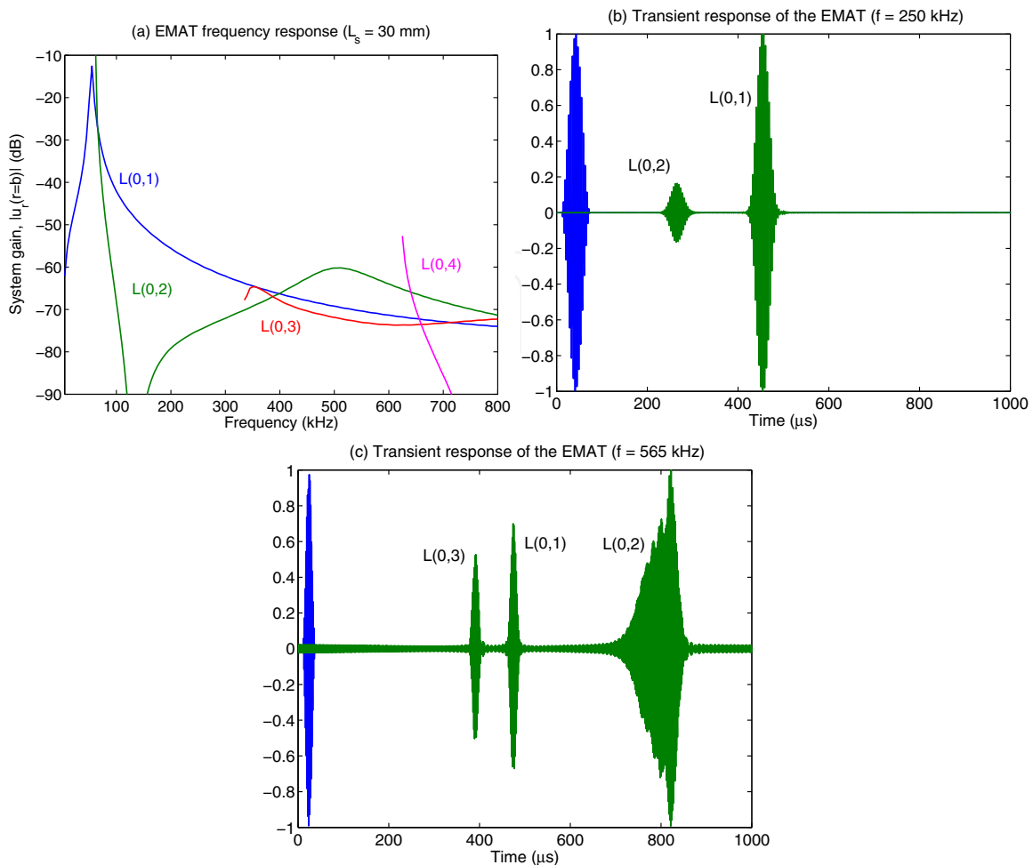
Fig. 9. (a) Computed frequency response of the EMAT for solenoid length L_s = 30 mm; transient waveforms at (b) 250 kHz and (c) 565 kHz. The signals in the transient plots have been normalized to unit amplitude.
