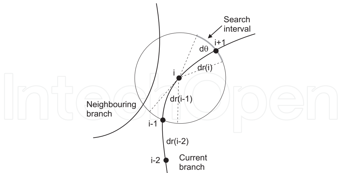
Fig. 4. Illustrates the root tracing algorithm used by PCDISP.
