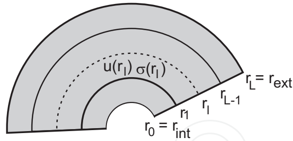
Fig. 2. Partition of the waveguide's cross section for solving the large fd problem.
