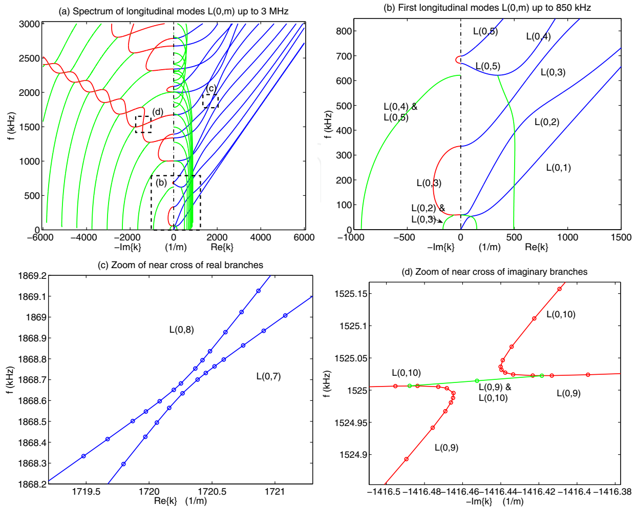
Fig. 3. Wavenumber-frequency plot for the L(0,m) modes of the aluminum pipe of table 6, for frequencies up to 3 MHz (part a). Part b shows the low-frequency spectrum, and the labelling scheme for the modes. Parts c and d show near crosses of the branches of two different modes; they have to be largely magnified to be visible.
