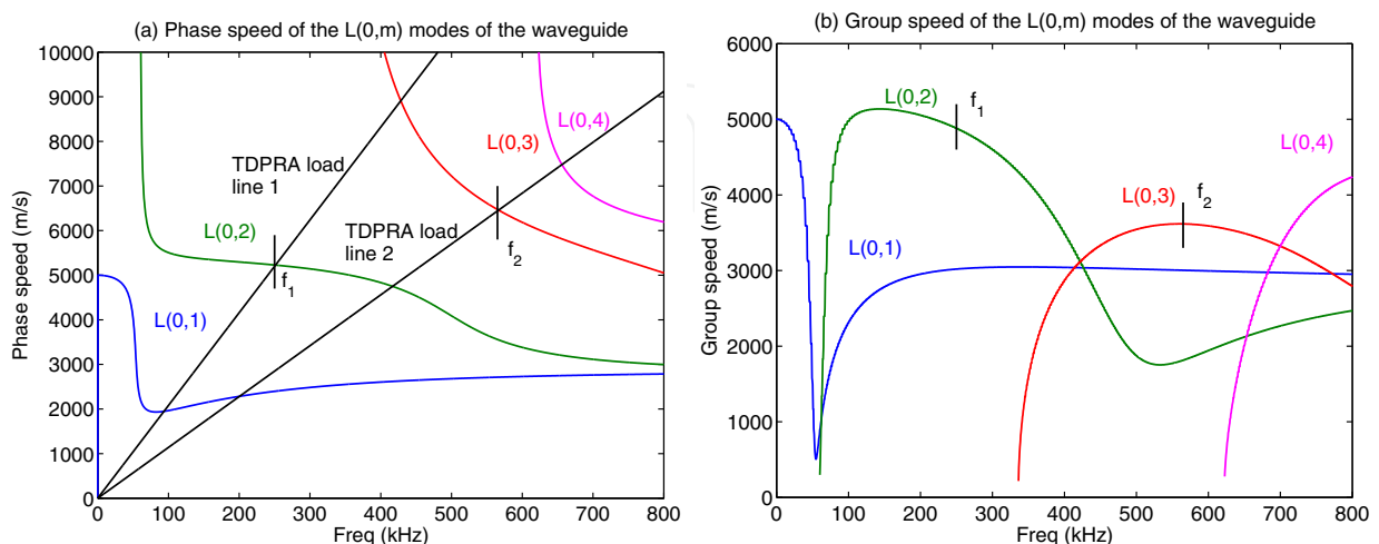
Fig. 7. (a) Phase and (b) group speeds of the first axisymmetric modes of the waveguide of table 6.
