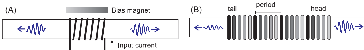
Fig. 6. Transducers used for generation of ultrasonic waves in cylindrical waveguides: (a) Electromagnetic Acoustic Transducer (EMAT) for Lorentz force excitation; (b) Time-Delay Periodic Ring Array (TDPRA) for piezoelectric excitation.
