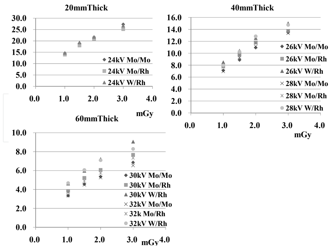
Fig. 5. CNR Analysis: 20mm, 40mm, and 60mm Thick PMMA Phantoms in System B.
