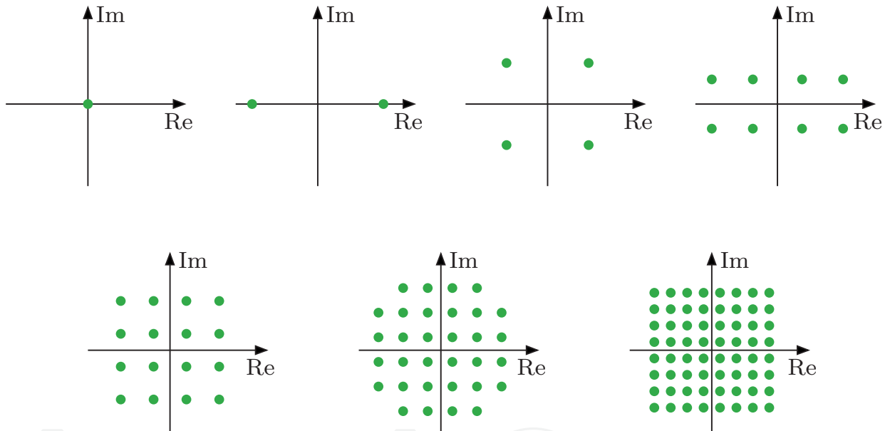
Fig. 3. QAM signal constellations: no modulation, BPSK, 4QAM, 8QAM, 16QAM, 32QAM, 64QAM
