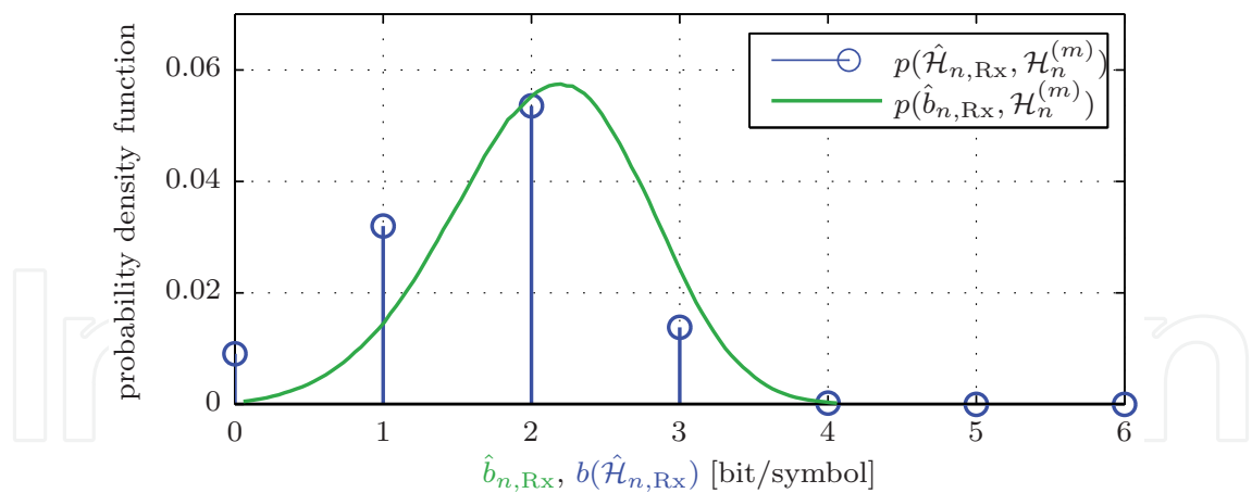
Fig. 9. Example of simulated probability density functions p(\hat{b}_{n,Rx}, \mathcal{H}_n^{(m)}) and p(\hat{\mathcal{H}}_{n,Rx}, \mathcal{H}_n^{(m)}) for b(\mathcal{H}_n^{(m)}) = 2 \text{ bit/symbol} and \gamma = 10 \text{ dB} ; the average bandwidth efficiency is 4 bit/symbol
