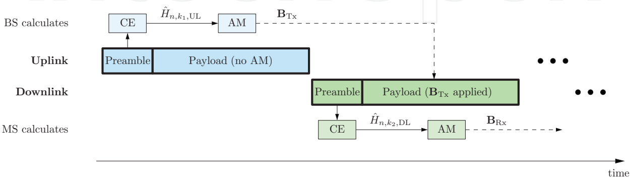
Fig. 5. TDD system structure
