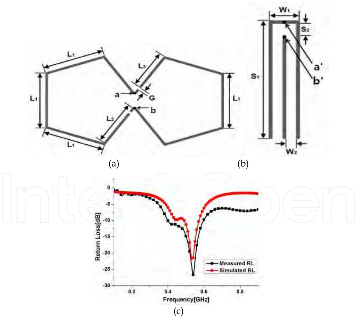
Fig. 13. Receiver antenna with buffer layer (Park, S. et al., 2008): (a) the pentagon dual loop antenna; (b) feeding structure; (c) simulated and measured return losses.
