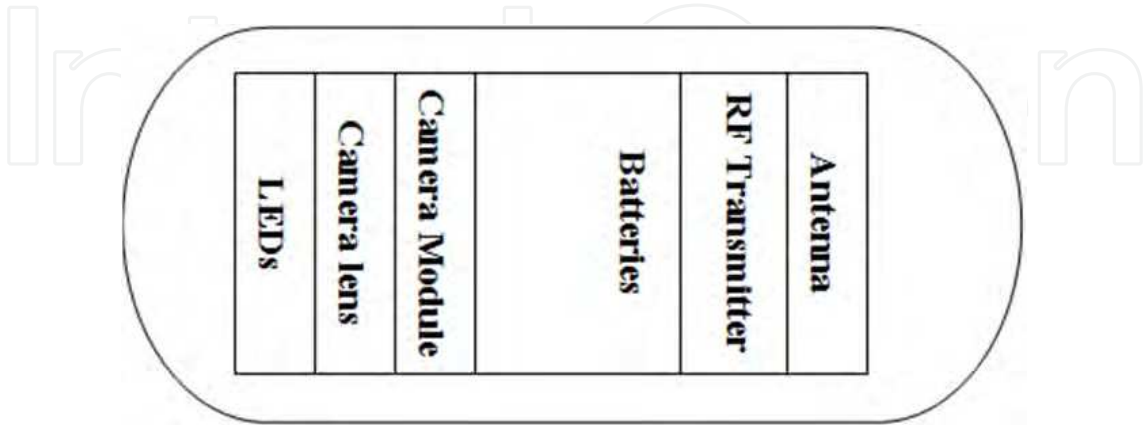
Fig. 2. Conceptual diagram of the WCE.
