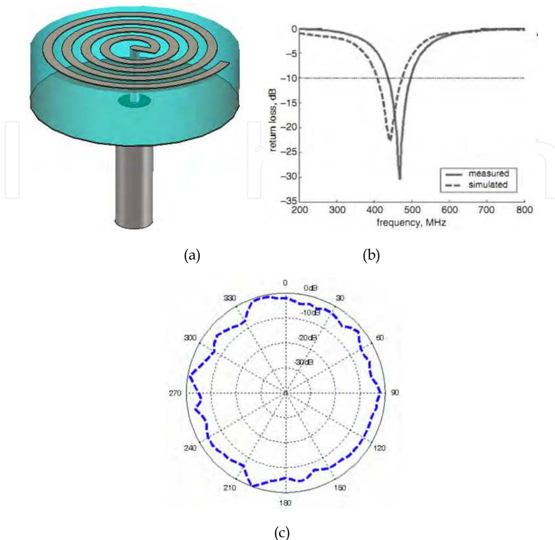
Fig. 3. Single arm spiral antenna (Kwak et al. 2005): (a) the geometric structure; (b) simulated and measured return losses; (c) azimuth pattern at 430MHz.
