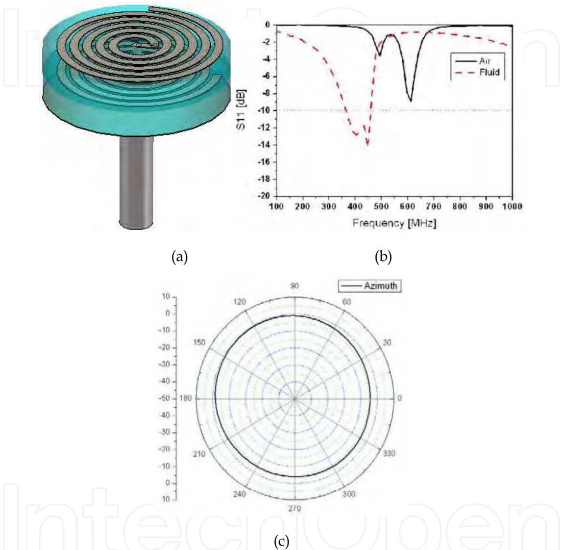
Fig. 4. Dual arm spiral antenna (Lee et al. 2007): (a) the geometric structure; (b) measured return losses; (c) azimuth pattern at 400MHz.
