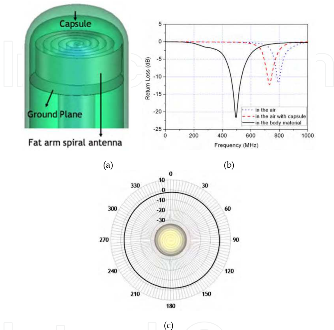
Fig. 6. Fat arm spiral antenna (Lee et al. 2010): (a) the geometric structure; (b) return losses; (c) azimuth pattern at 450MHz.
