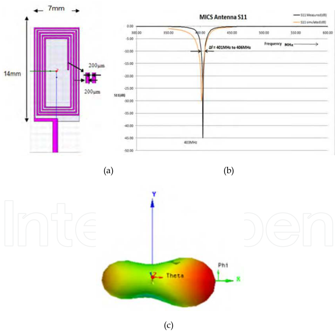
Fig. 11. Rectangular microstrip loop antenna (Shirvante et al. 2010): (a) the geometric structure; (b) simulated and measured return losses; (c) azimuth pattern at 403MHz.
