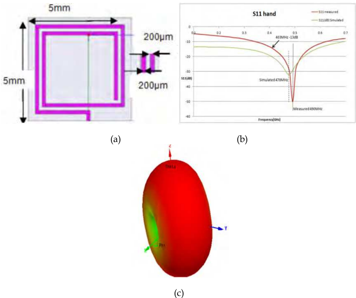
Fig. 7. square microstrip loop antenna (Shirvante et al. 2010): (a) the geometric structure; (b) simulated and measured return losses; (c) azimuth pattern at 403MHz.
