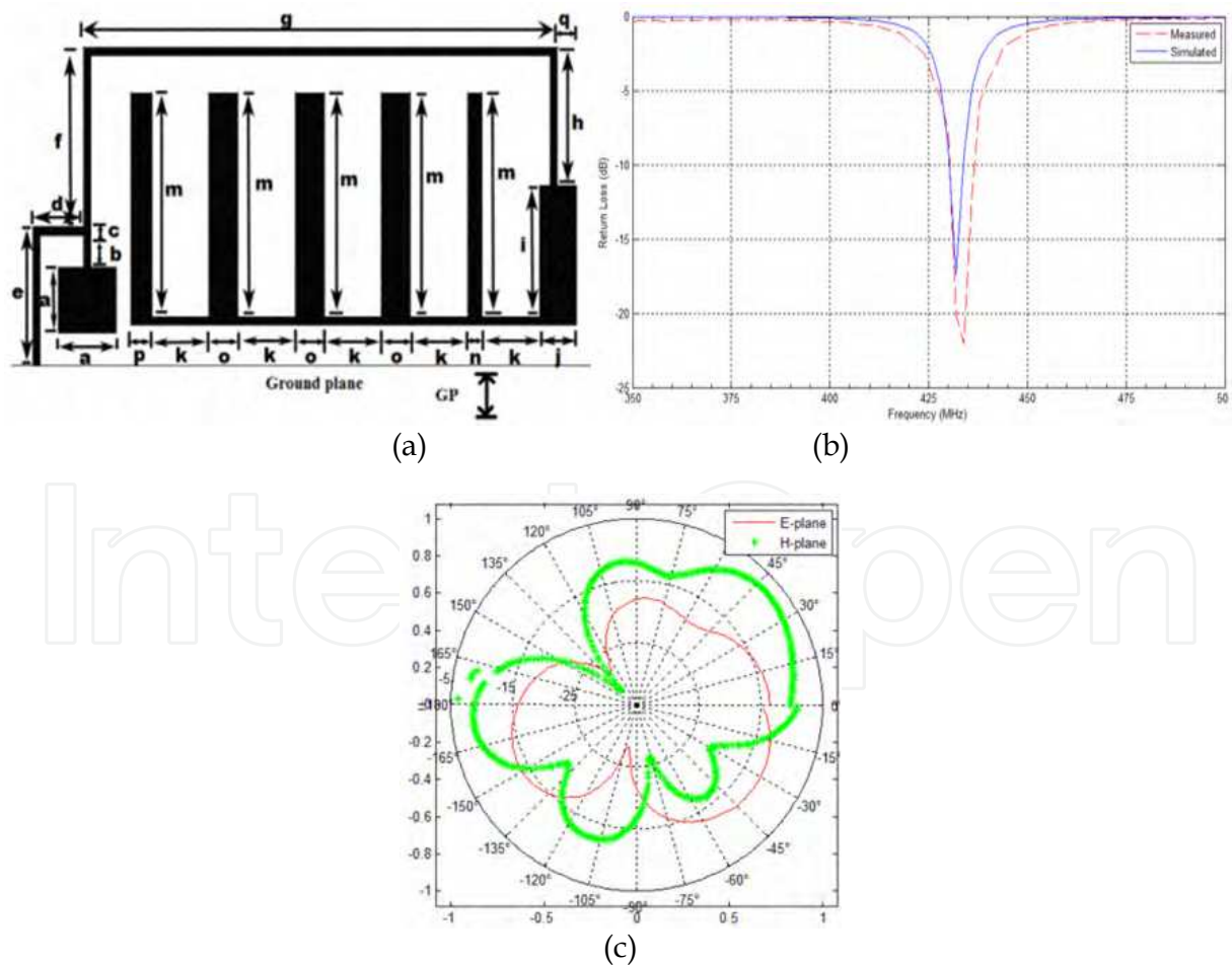
Fig. 12. Microstrip planar antenna (Babar et al. 2009): (a) the geometric structure; (b) simulated and measured return losses; (c) radiation patterns at 433MHz.
