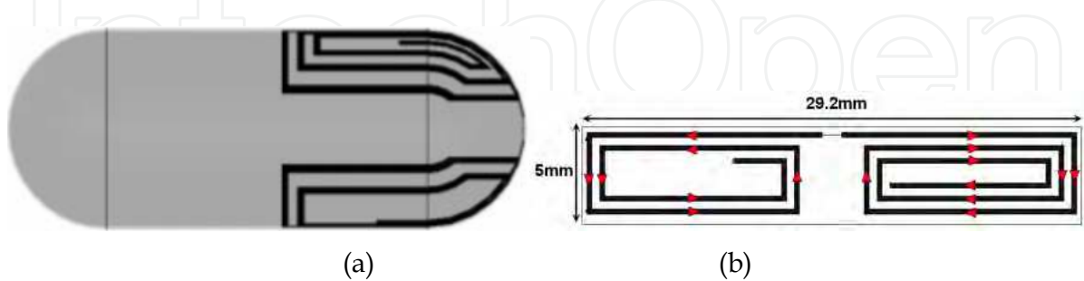
Fig. 8. Conformal chandelier meandered dipole antenna (Izdebski et al., 2009): (a) the geometric structure of the conformal chandelier meandered dipole antenna; (b) Offset Planar Meandered Dipole Antenna with current alignment vectors.
