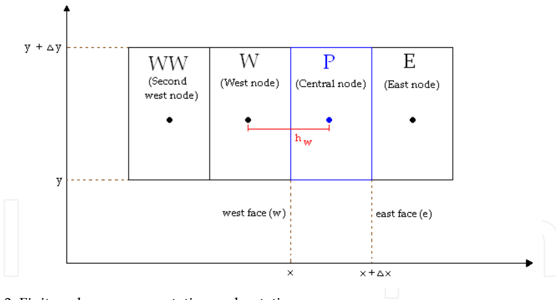
Fig. 3. Finite volume representation and notation.
