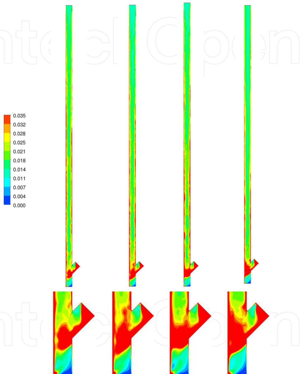
Fig. 8. Solids volumetric fraction in the center of the riser. Simulation time 15 sec. Left to right: LES Smagorinsky, LES WALE, LES Dynamic model, Detached Eddy Simulation (DES).
