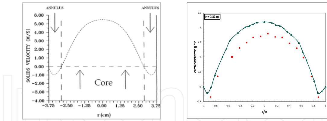
Fig. 6. Comparison of solid phase velocity profile presented by Miller and Gidaspow (1992) with the CFD simulations (-▲-) and experimental data performed by Samuelsberg and B. H. Hjertager (1996) (●).
