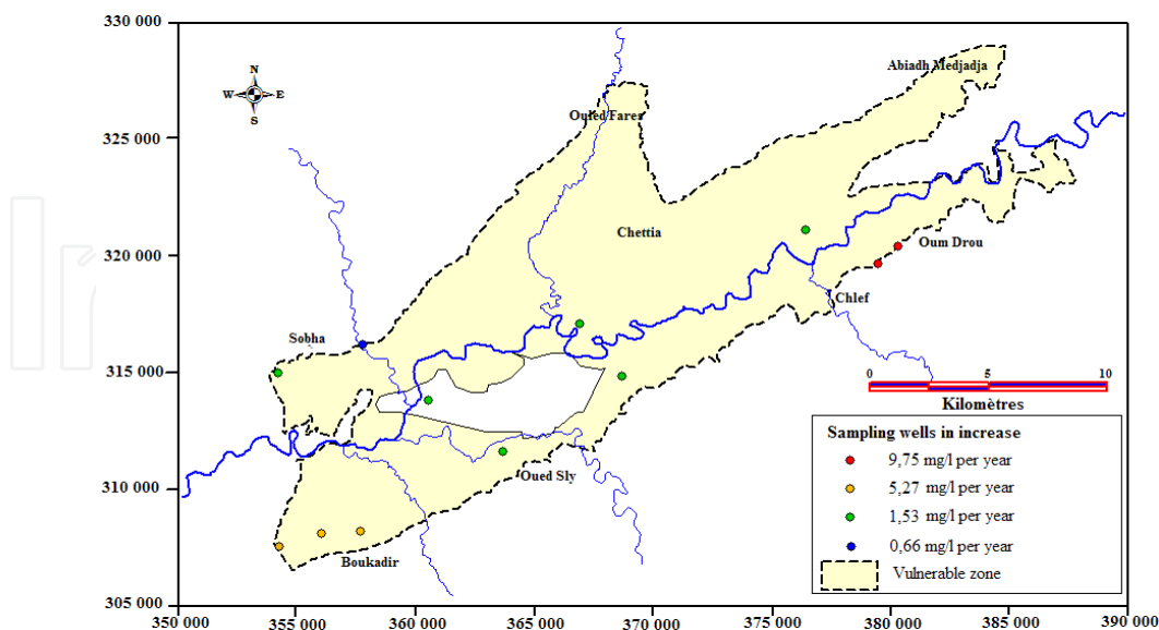
Fig. 6. Specific evolution of the contents nitrates wells in increase (1992-2004)
