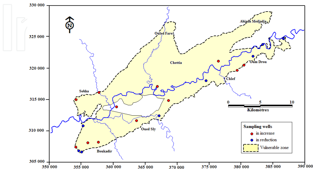
Fig. 5. Evolution of the contents from 1992 to 2004
