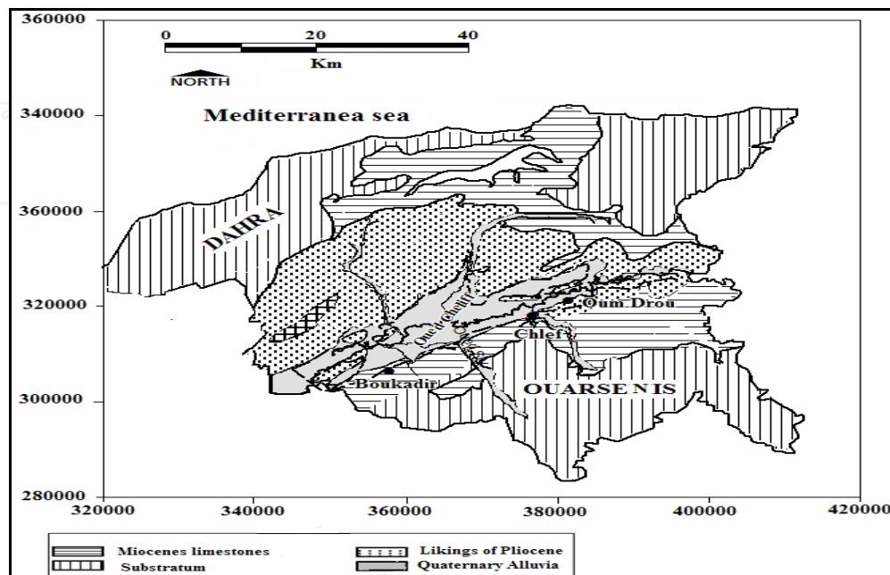
Fig. 2. Geological context of study area (Perrodon (1957) & Mattauer (1958))
