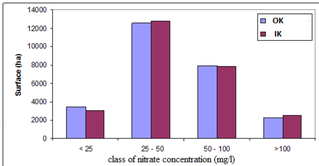
Fig. 10. Comparison between the surfaces of \text{NO}_3 classes gotten by OK and IK methods
