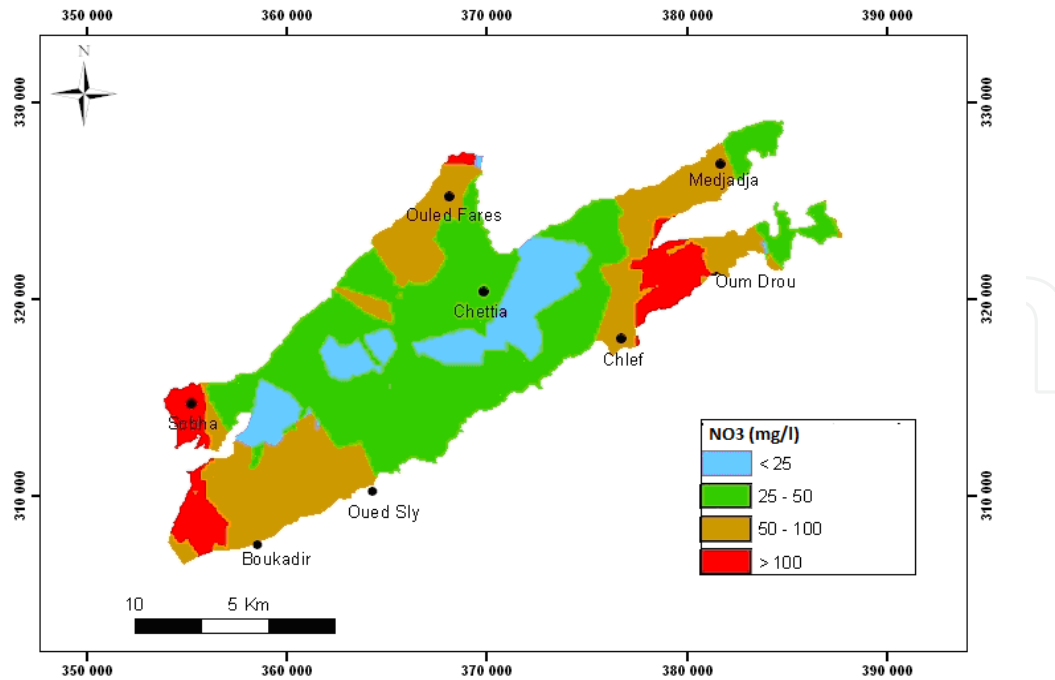
Fig. 9. Map of nitrate concentrations estimated by Indicator kriging (IK) method
