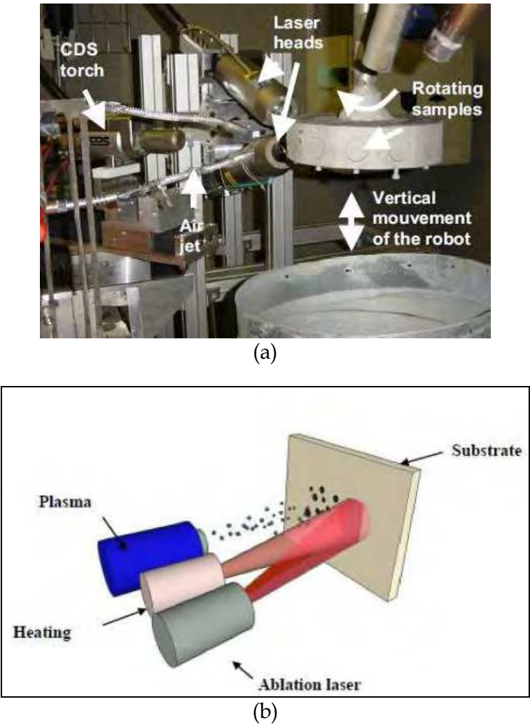
Fig. 4. (a) PROTAL® coupled to HVOF gun by Costil et al. (Costil et al., 2004a) (b) Two Nd-YAG lasers coupled with a plasma spray gun by Danlos et al. (Danlos et al., 2011)
