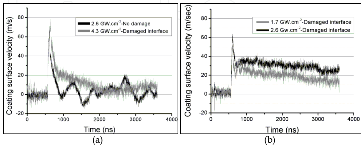
Fig. 20. Velocity profiles of cold-sprayed Al surface on (a) as- received AISI 2017 substrate (b) laser pre-treated (2.2 J.cm -2 ) substrate AISI 2017
