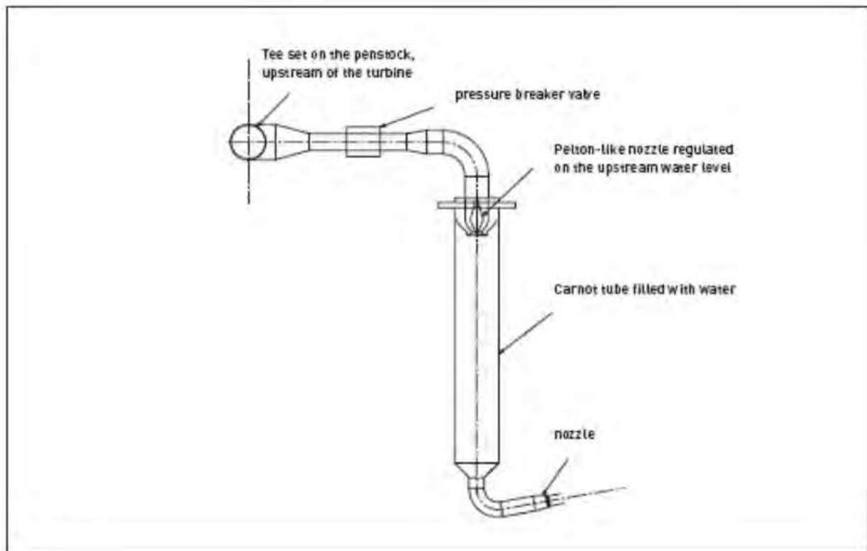
Fig. 8. Carnot pressure breaker.
