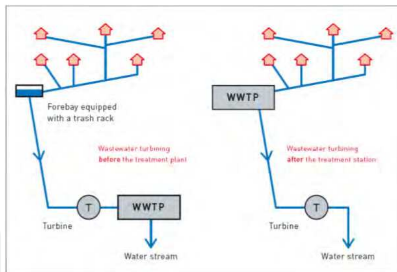
Fig. 3. Turbine setting before and after the wastewater treatment plant (WWTP).
