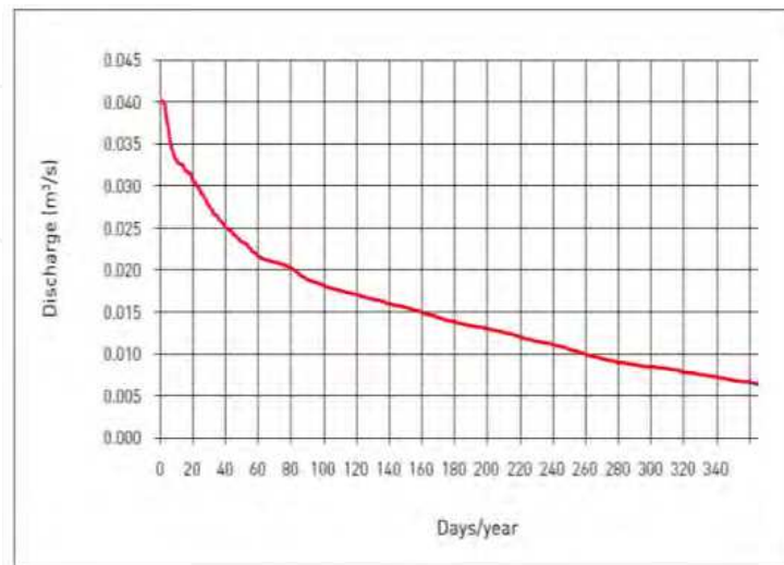
Fig. 4. Example of a flow duration curve.
