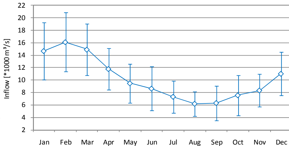
Fig. 1. Average and standard deviation of monthly inflows for the Itaipú hydro plant.
