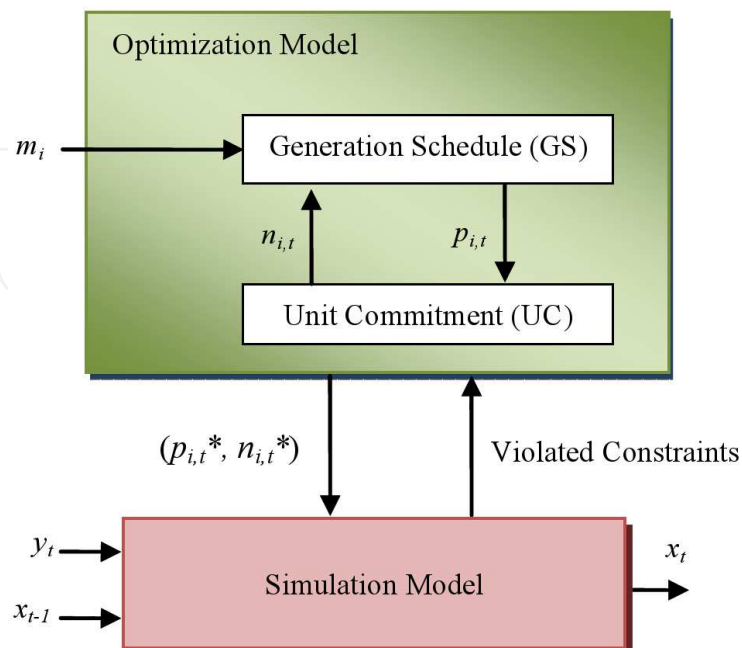
Fig. 7. Relaxation approach for solving the STHS problem.
