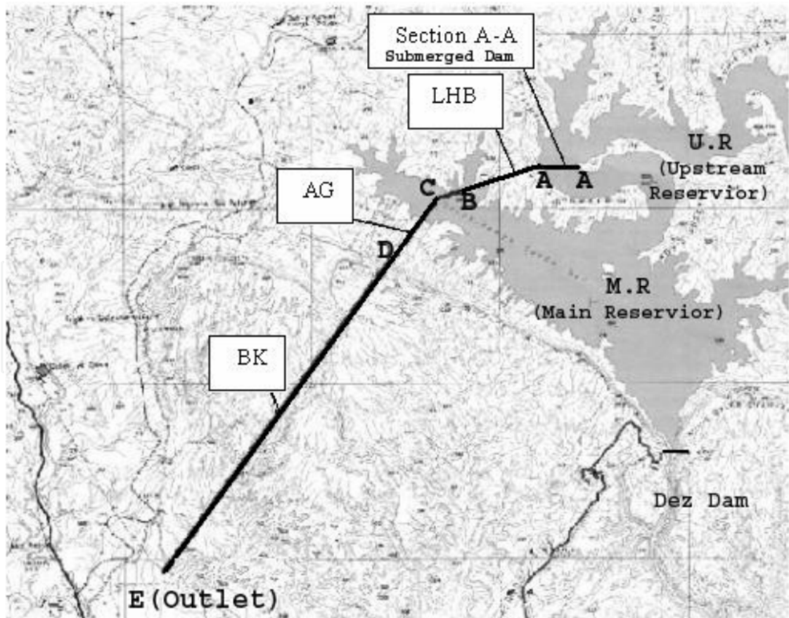
Fig. 13. Layout of diversion tunnel (path ABCDE).
