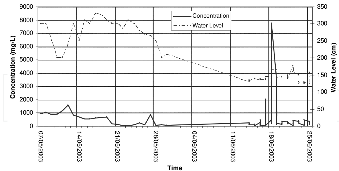
Fig. 12. Sediment concentration and water levels for Dez-Harmaleh.
