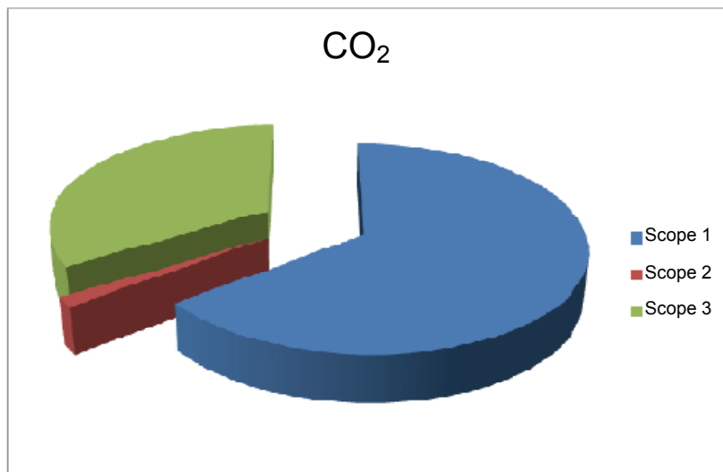
Fig. 2. Overall Brock University GHG (Carbon) Footprint Chart (Adapted from Mitchell and Parmar, 2010)
