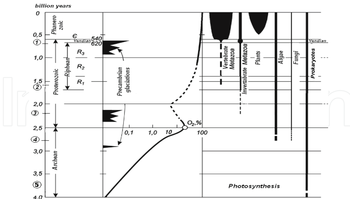
Fig. 2. The main events in early biosphere history (by Rozanov, 1986). In center: changes of the atmospheric oxygen concentration. On the right: times of appearance of some main taxa are given by full lines; dotted lines give possible presence of the group, but are unconfirmed or indirectly confirmed. In circles left: 1 - Vendian phytoplanktonic crisis; 2 - appearance of first hypothetic pre-vertebrate organisms (by hypothesis of Rozanov, 1986); 3 - developed photosynthesizing communities, appearance of first multicellular animals (invertebrate); 4 - in the sediments of this period first eukaryotes have been found; appearance of first plants and fungi; 5 - period of appearance of prokaryotes and probably mechanism of photosynthesis. The "flags" mean periodic glaciations, which took place in Precambrian.
