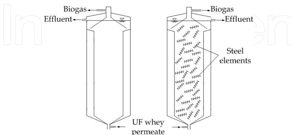
Fig. 1. Schematic of the laboratory-scale anaerobic treatment system
