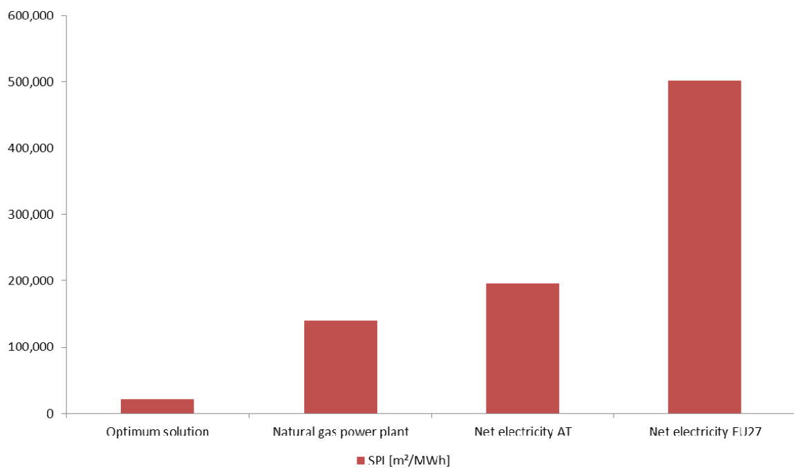
Fig. 7. Comparison of electricity production
