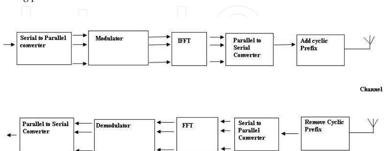
Fig. 1. OFDM system
