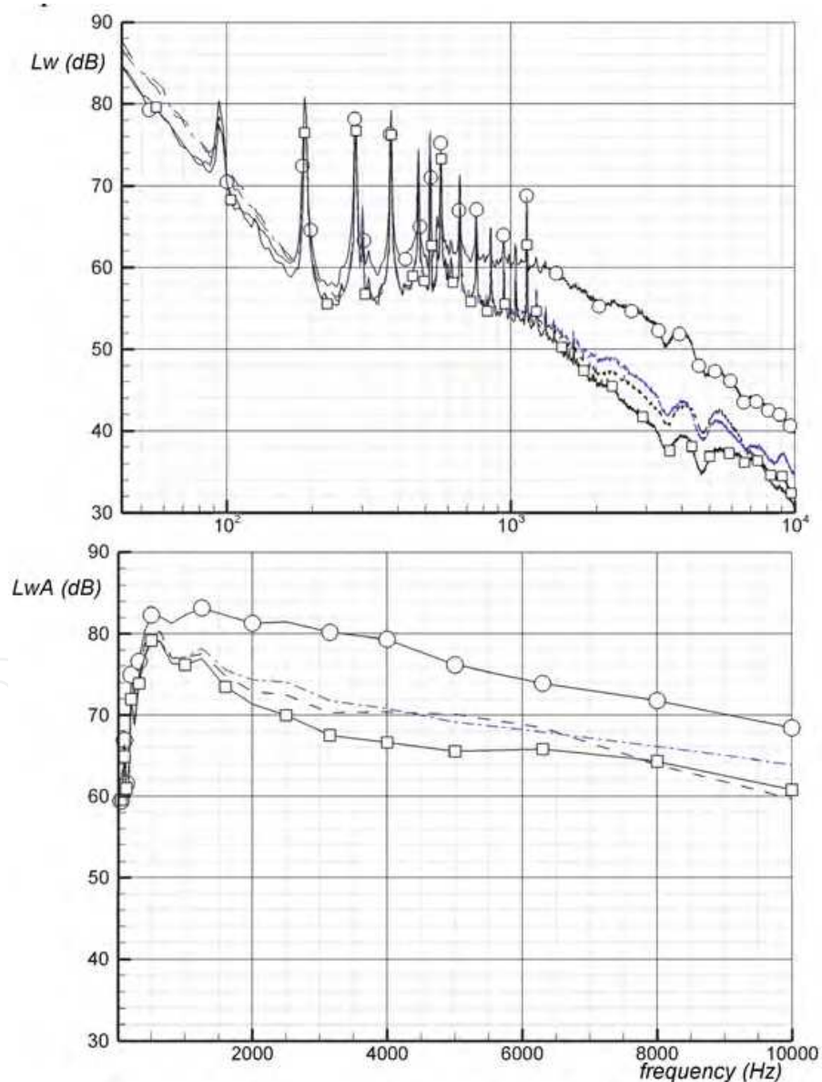
Fig. 7. Comparison of L_w (top) and L_wA (bottom) for the different blade geometries
