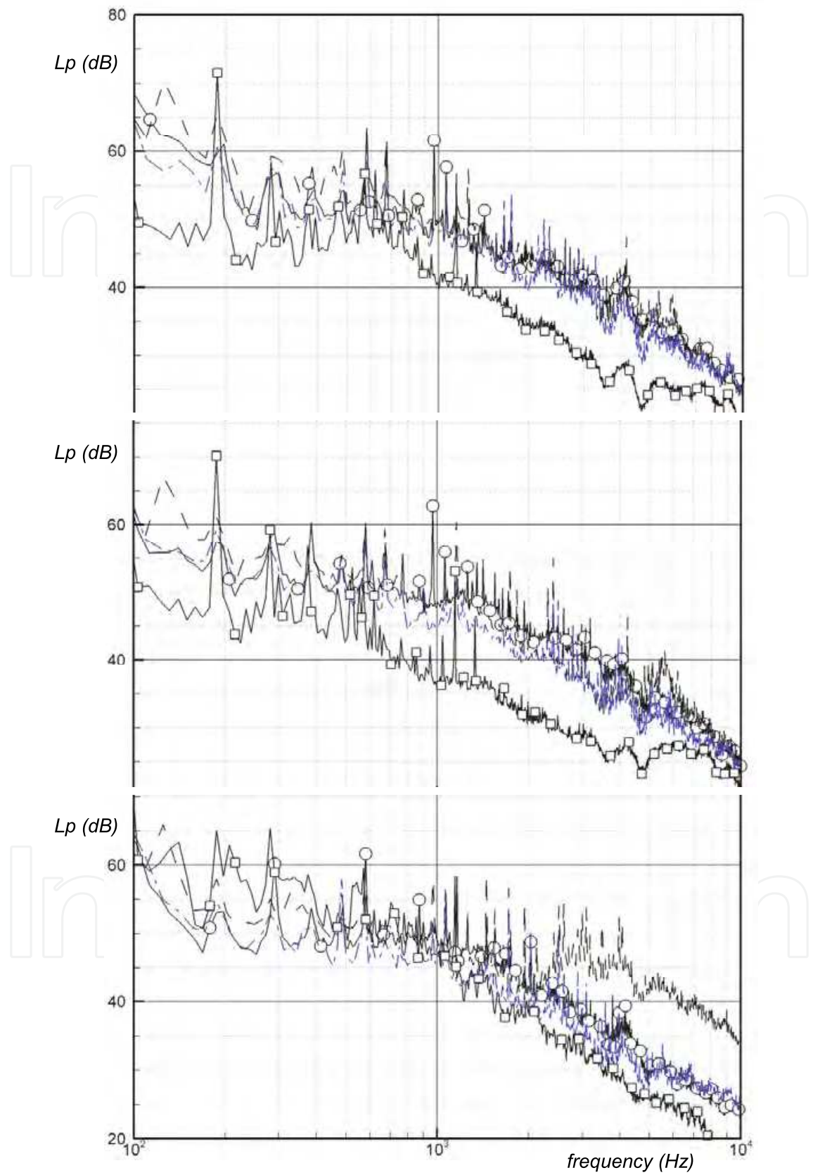
Fig. 6. Auto-spectra of the L_p for the different blade geometries at three azimuthal position: 30° (top), 60° (mid) and 90° (bottom)
