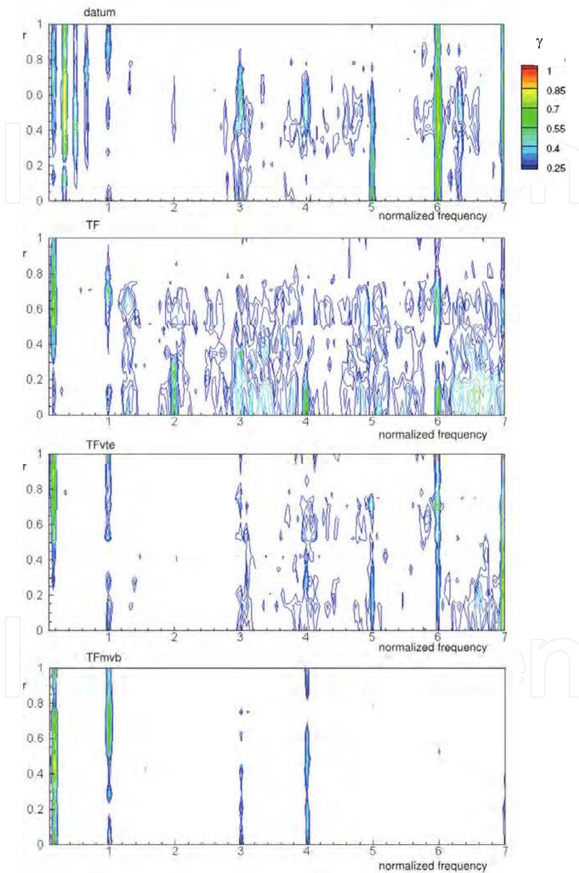
Fig. 10. Spanwise maps of coherence for the different blade geometries at 90^\circ
