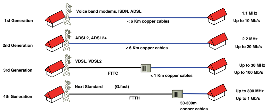
Fig. 1. Comparison of DSL Generations.
