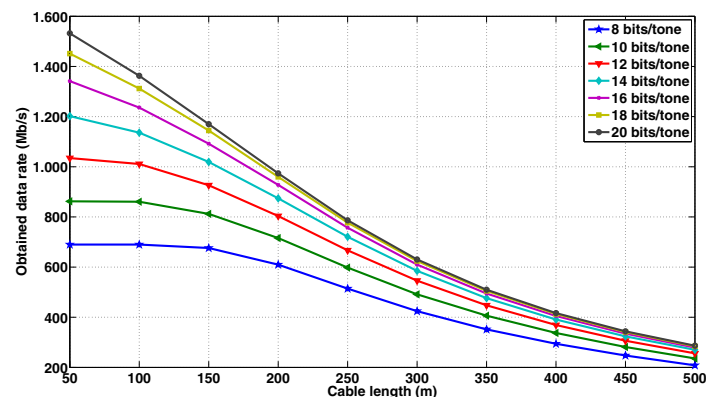
Fig. 23. Obtained data rates using different values of maximum number bits/tone. No crosstalk is taken into account. 0.4mm fitted cable model.
