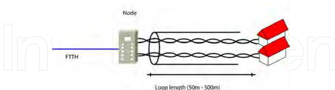
Fig. 20. Second scenario for evaluation of the achievable data rates of 4th generation DSL systems. Crosstalk is taken into account.
