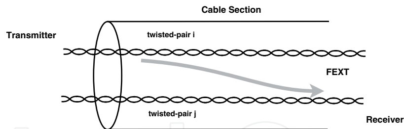
Fig. 4. Far-end crosstalk.
