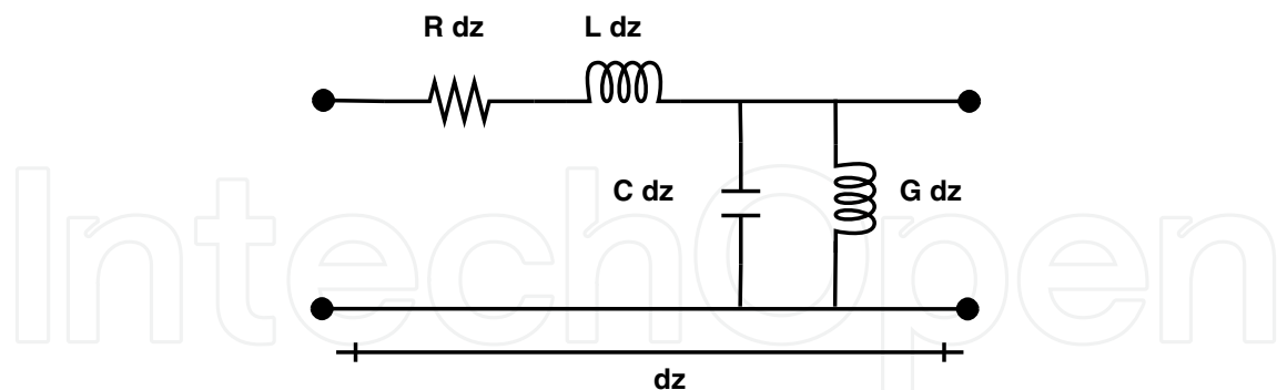
Fig. 2. Transmission line model per unit length dz .
