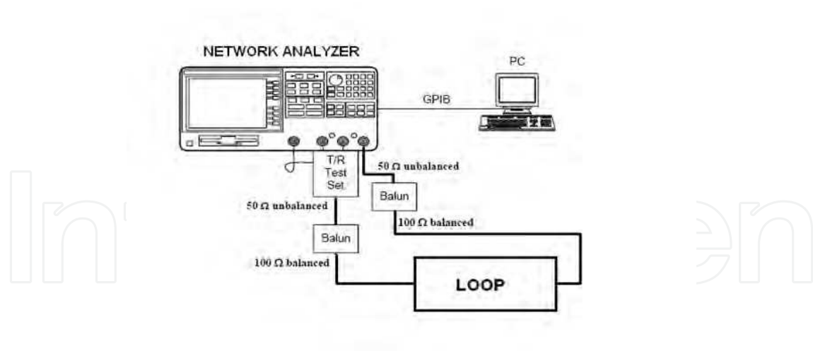
Fig. 6. Experimental setup used during the measurements campaign.
