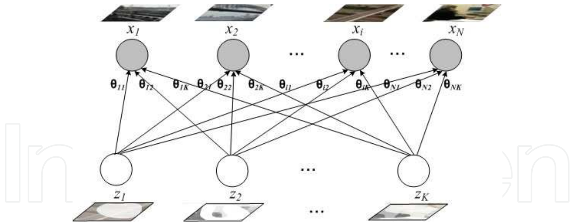
Fig. 8. In the probabilistic generative process of LDA, the observed data instances (documents) are represented as a mixture of hidden topics, and the topic mixture vector \theta determines how an instance x is mixed over K hidden topic localities. Note that after resetting of \theta in the above adaptive instance assignment, most connections between x and z will be of zero coefficients.
