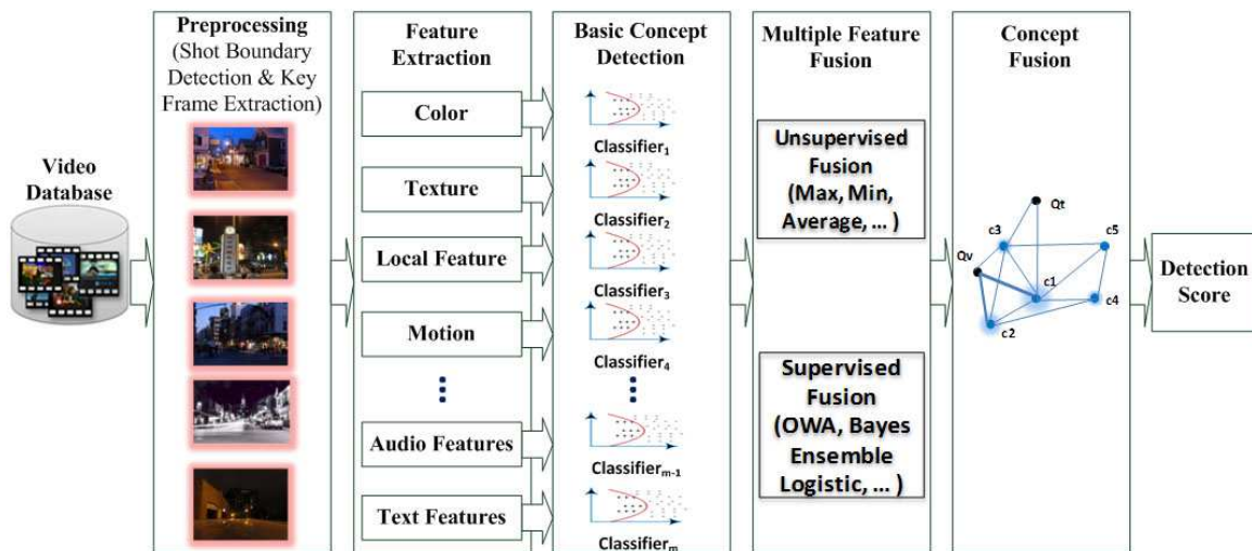
Fig. 3. General procedure of concept detection
