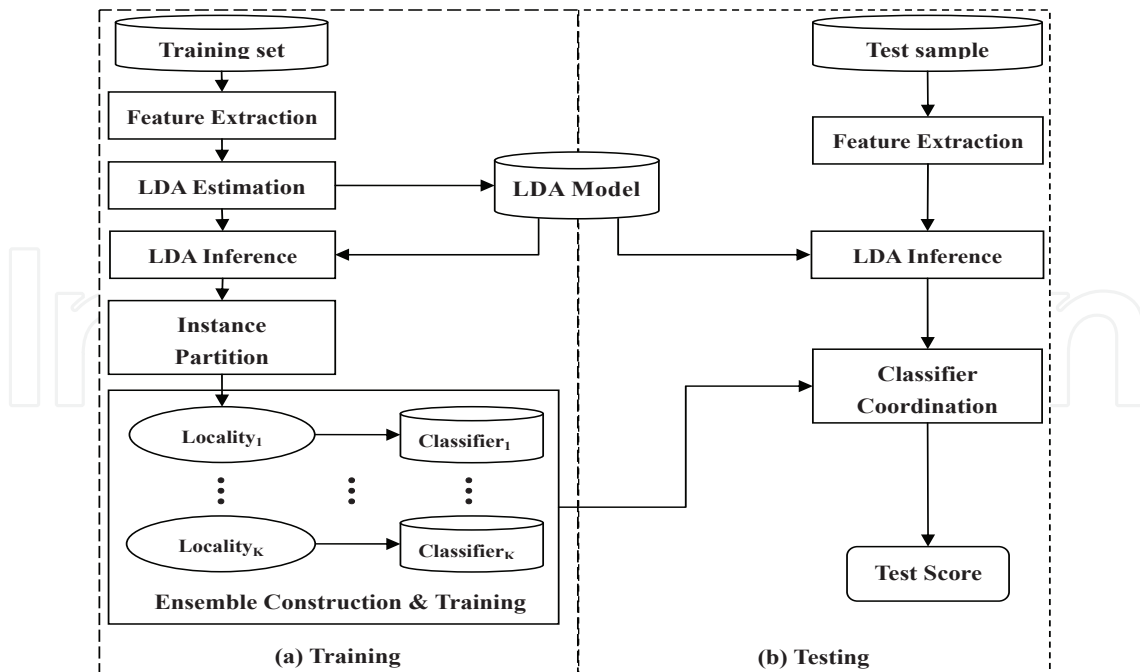
Fig. 5. The overall framework. The proposed ensemble first exploits LDA to represent data instances as a mixture of hidden topics and partition the data space into topic localities, and then coordinates the individual classifiers in each topic locality for final classification based on the topic mixture of LDA topics which is naturally achieved during LDA inference without additional classifier selection.
