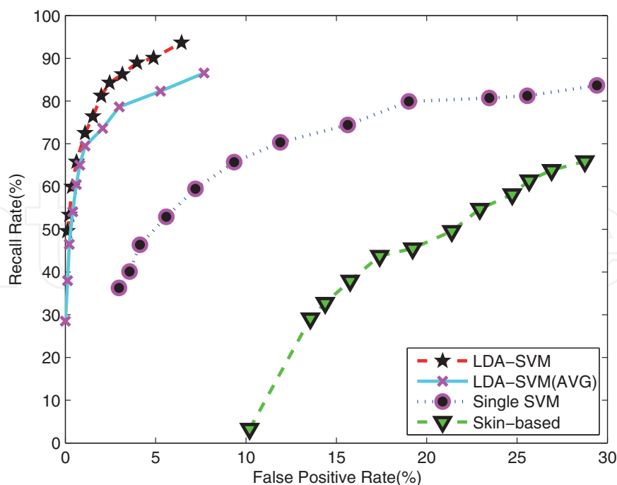
Fig. 11. ROC Curves for Pornography Detection
