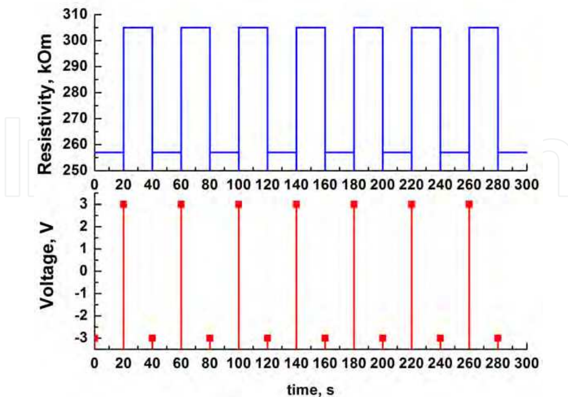
Fig. 21. Two state resistive switching of the ZnO nanowire device at RT. Applied voltage versus time (lower curve); readout resistance versus time (upper curve).
