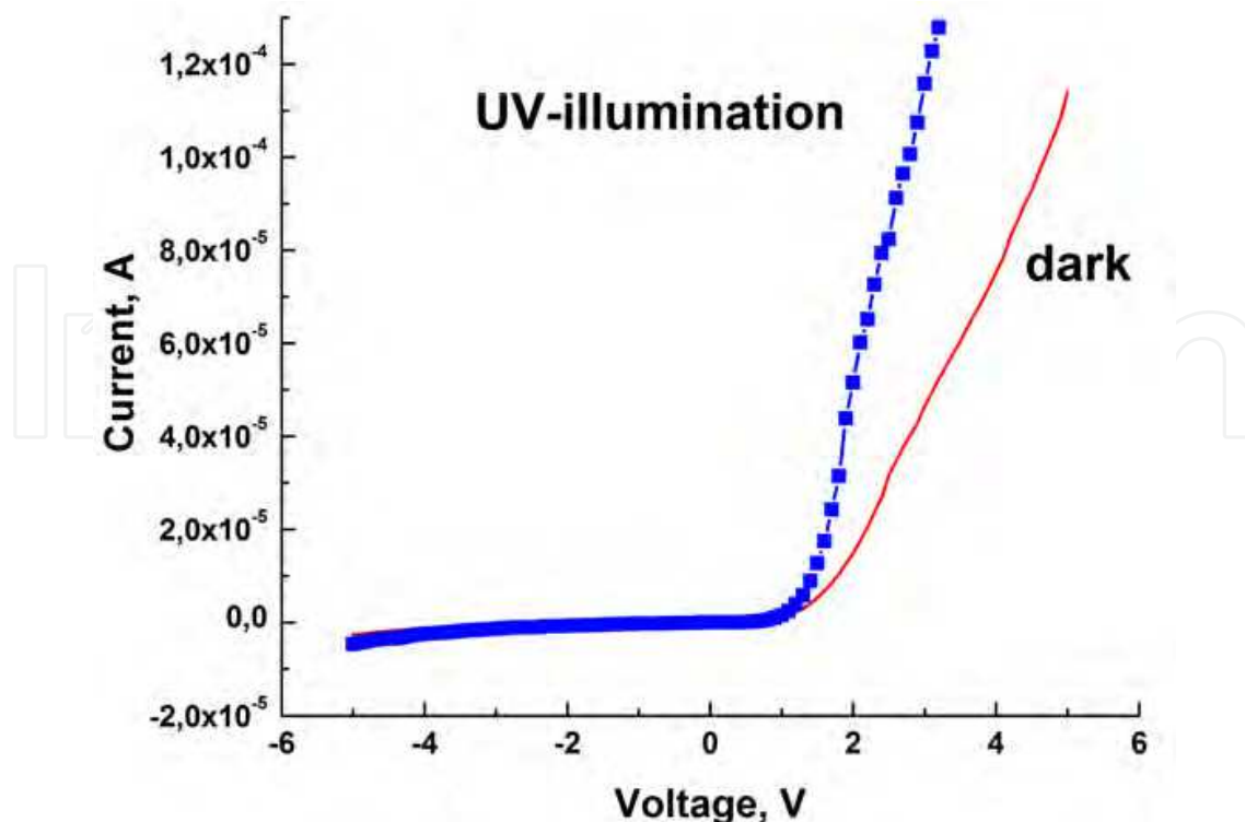
Fig. 13. Typical I-V characteristics of a pn-heterojunction diode under dark and UV-illumination conditions at room temperature. The threshold voltage is \sim 1.5 V.
