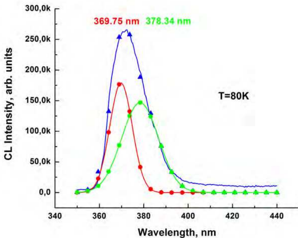
Fig. 9. CL spectrum of medium-time annealed Sb-doped ZnO nanorod arrays grown on n + -Si (100) substrate.
