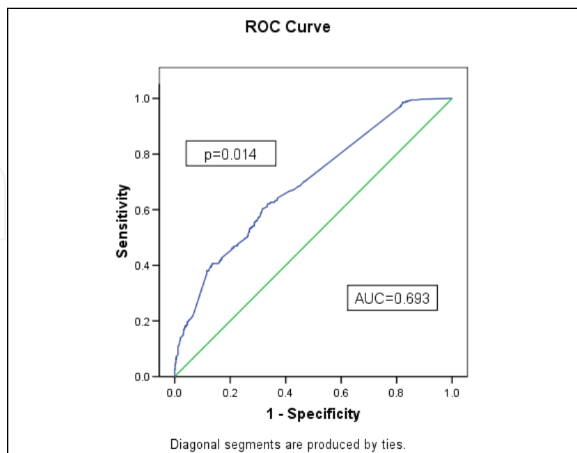
Fig. 3. ROC curve, based on sensitivity and specificity of the multivariable model, with traditional risk factors and without GRS.
