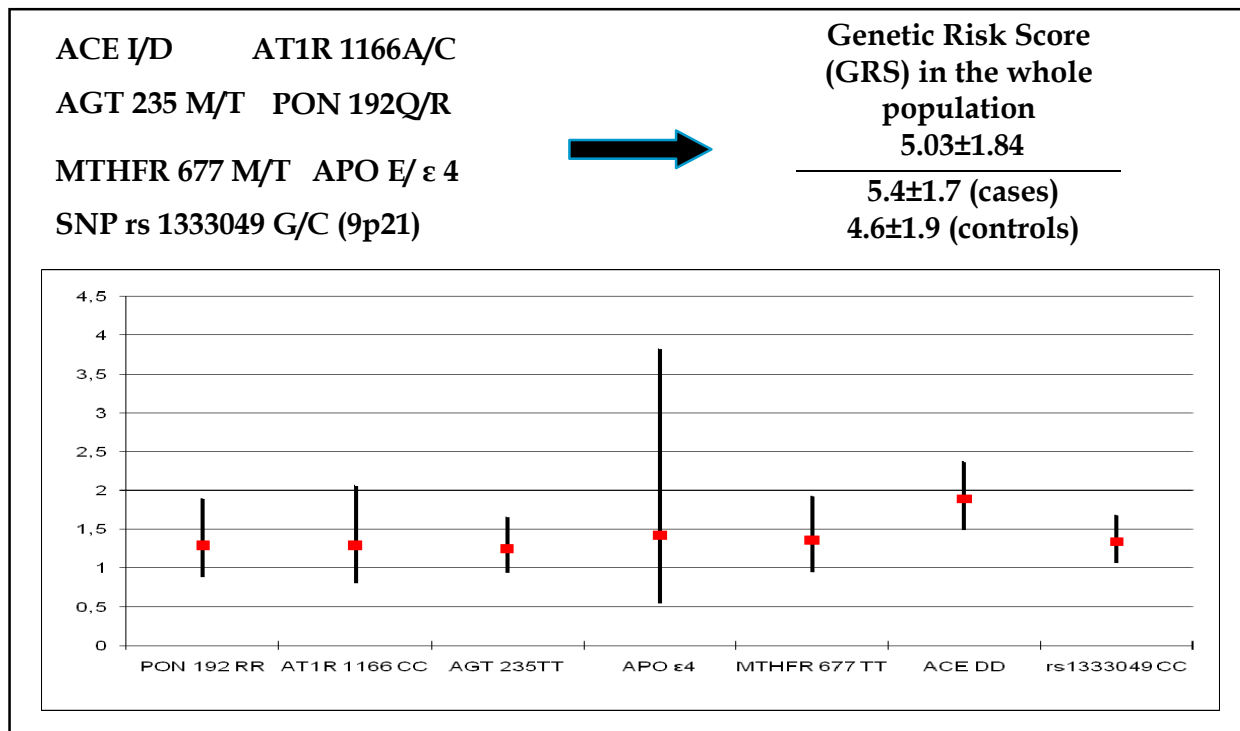
Fig. 1. CHD genetic risk (OR) conferred by each isolated polymorphism and the GRS obtained by the addition of all the 7 risk alleles of the studied variants.
