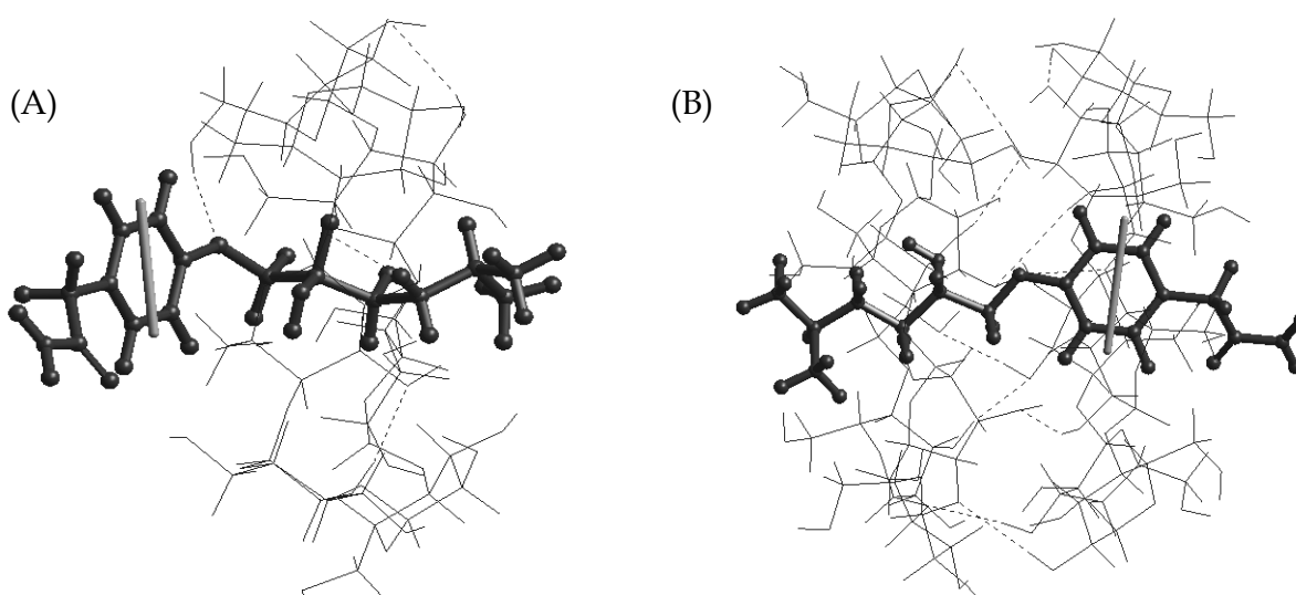
Fig. 17. Proposed structures for the (A) 1:1 and (B) 1:2 atenolol- \beta -CD inclusion complexes, via molecular modeling. The dotted lines represent hydrogen bonds. The transition moment of atenolol is plotted in grey.
