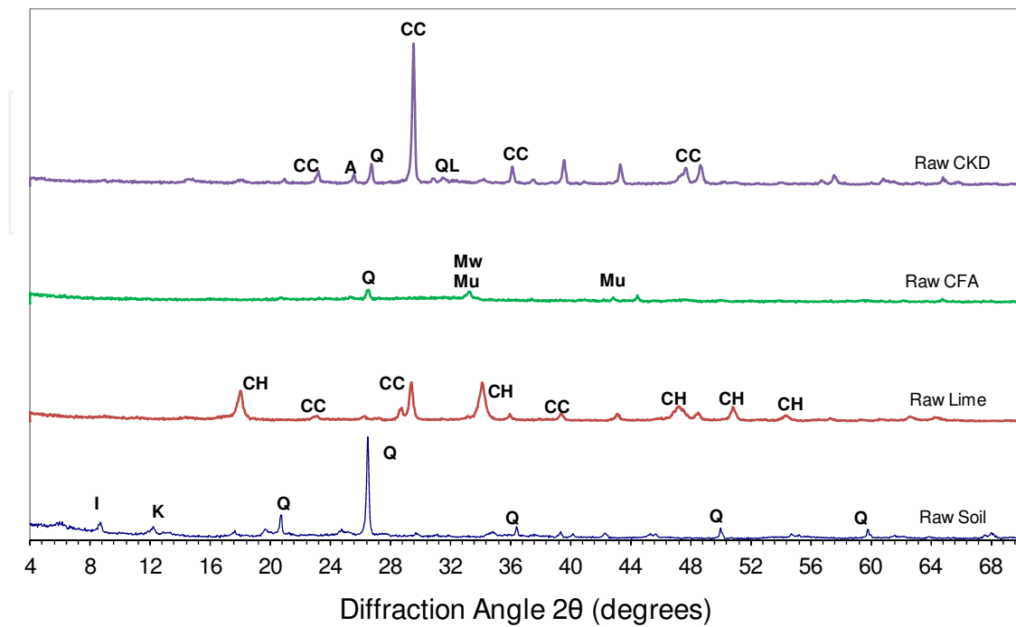
Fig. 9. XRD pattern for raw soil, lime, CFA and CKD powders [CC-calcite ( \text{CaCO}_3 ), A-anhydrite ( \text{CaSO}_4 ), QL-quicklime ( \text{CaO} ), Q-quartz ( \text{SiO}_2 ), Mu-mullite ( \text{Al}_6\text{Si}_2\text{O}_{13} ), Mw-merwinite ( \text{Ca}_3\text{Mg}(\text{SiO}_4)_2 ), CH-calcium hydroxide ( \text{Ca}(\text{OH})_2 ), I-illite, K-kaolinite)
