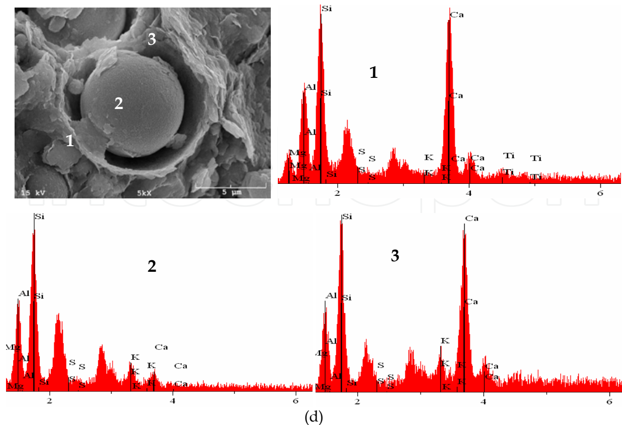
Fig. 7. (Cont'd). SEM/EDS of 28-Day Cured 15% CFA-Stabilized Caranasaw Soil Specimens (d) reaction shell of CFA particle
