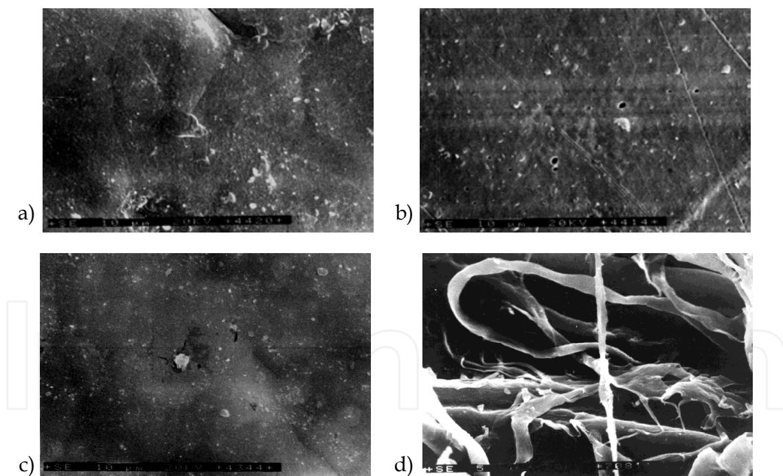
Fig. 10. SEM micrographs of 40/60 composition after a) photodegradation b) thermodegradation c) photothermodegradation d) hydrolysis
