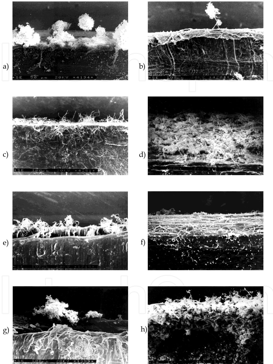
Fig. 5. SEM micrographs of neat 70/30 composition after biodegradation with a) Aspergillus niger b) Aspergillus terreus c) Paecilomyces varioti d) Penicillium funiculosum e) Penicillium ochrocloron f) Scopulariopsis brevicaulis g) Trichoderma viride h) mixed fungal population
