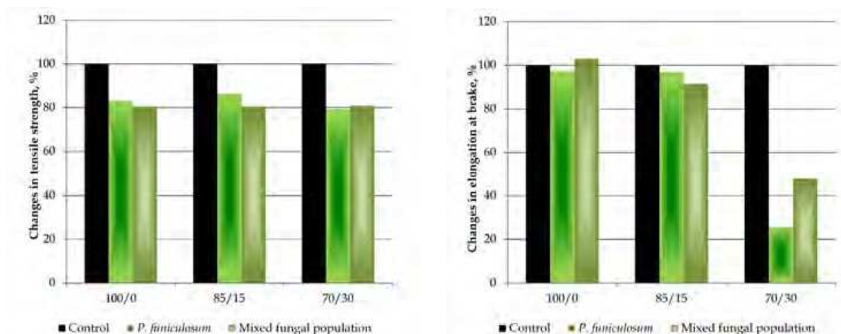
Fig. 1. Mechanical properties of films after biodegradation
