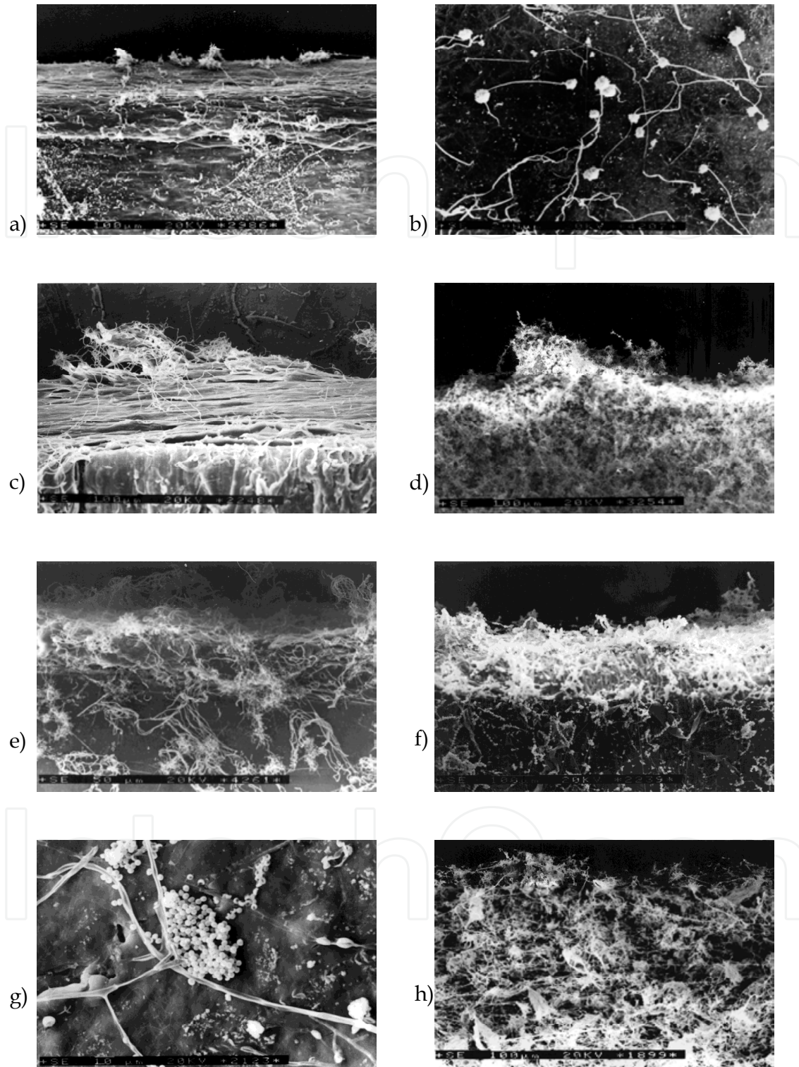
Fig. 6. SEM micrographs of neat 40/60 composition after biodegradation with a) Aspergillus niger b) Aspergillus terreus c) Aureobasidium pullulans d) Penicillium funiculosum e) Penicillium ochrochloron f) Scopulariopsis brevicaulis g) Trichoderma viride h) mixed fungal population
