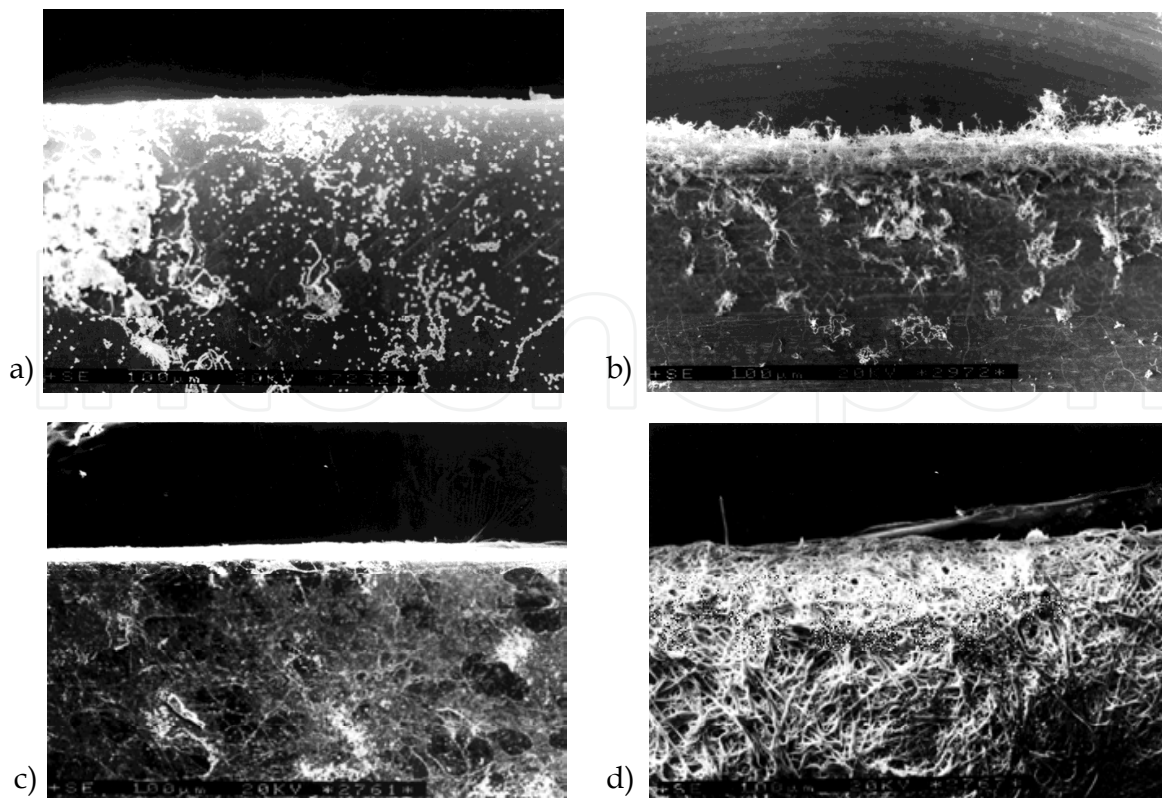
Fig. 12. SEM micrographs of films after exposing to different abiotic factors and subsequent biodegradation with mixed fungal population a) LDPE after thermo- and biodegradation b) 85/15 composition after photo- and biodegradation c) 70/30 composition after photo-thermo- and biodegradation d) 40/60 composition after hydrolysis and biodegradation
