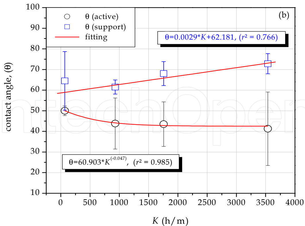
Fig. 9. Relationships of surface roughness (a) and wettability (b) to internal fouling
