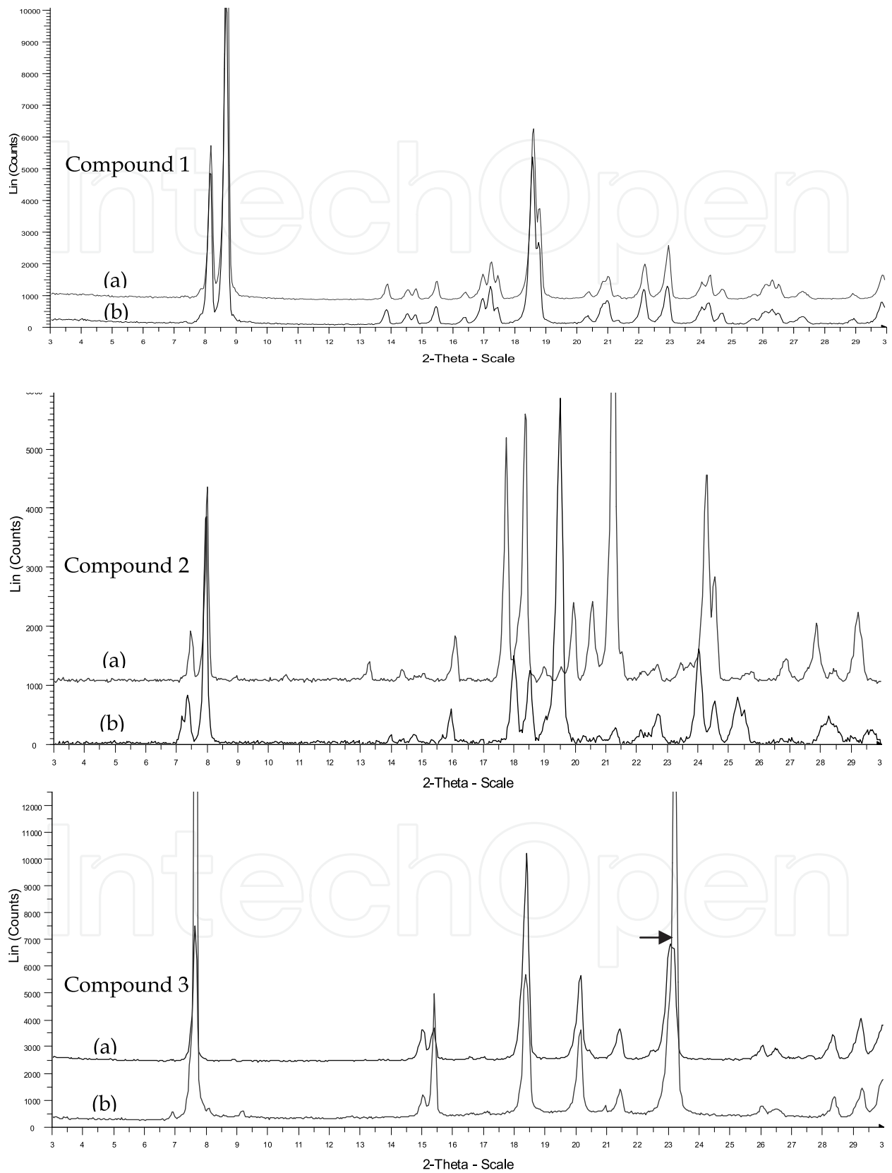
Fig. 15. Comparison of X-Ray patterns for the detection of conglomerate
