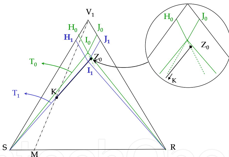
Fig. 6. Principle of crystallization by entrainment
