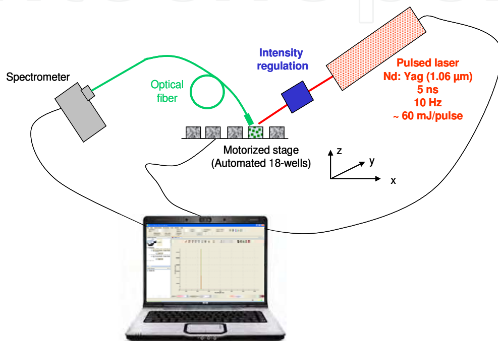
Fig. 11. Experimental Set-up
