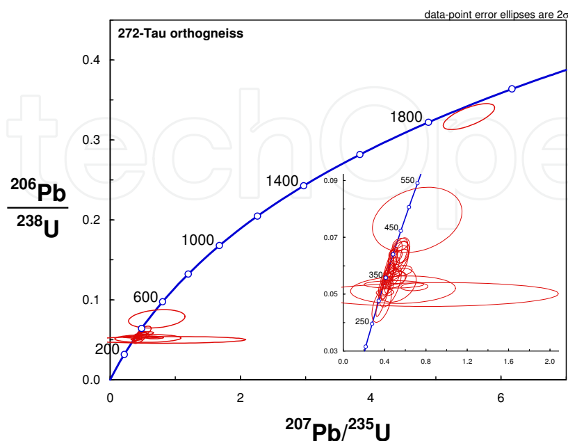
Fig. 18. Concordia projection for sample 272.
