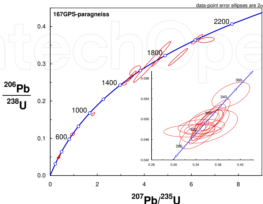
Fig. 20. Concordia projection for sample 167GPS.
