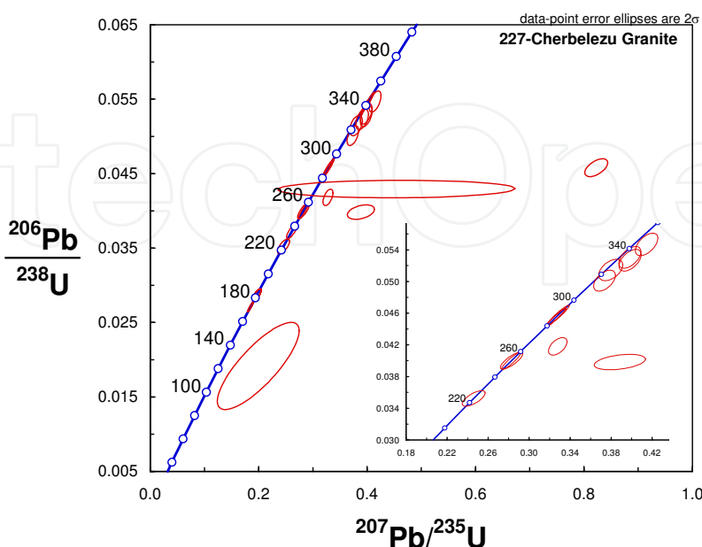
Fig. 3. Concordia projection for sample 227.
