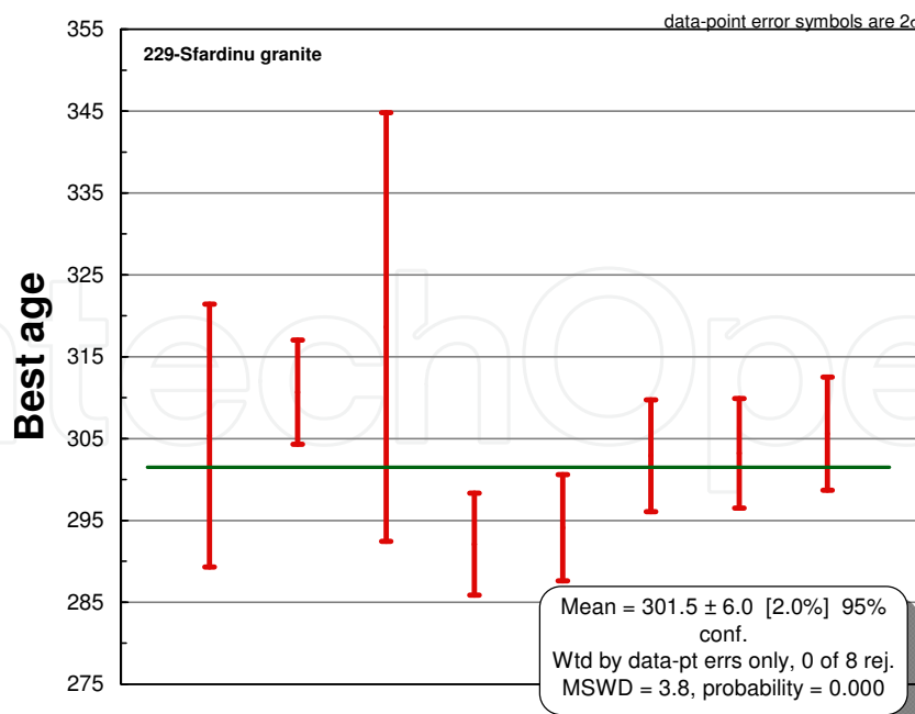
Fig. 5. Weighted mean age for sample 229.
